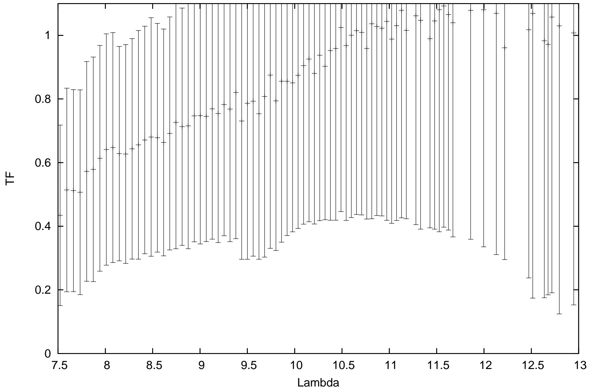
calHD123139_flux-0.39_diam5.34_r.MIDI.2011-04-08T02_08_17.000_K011
