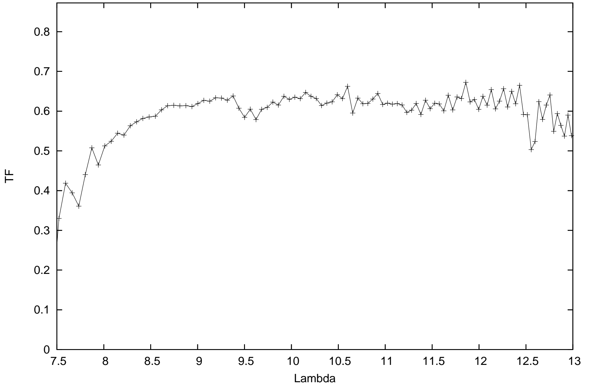
calHD123139_flux-0.39_diam5.34_r.MIDI.2011-05-10T01_55_39.000_D0B2
