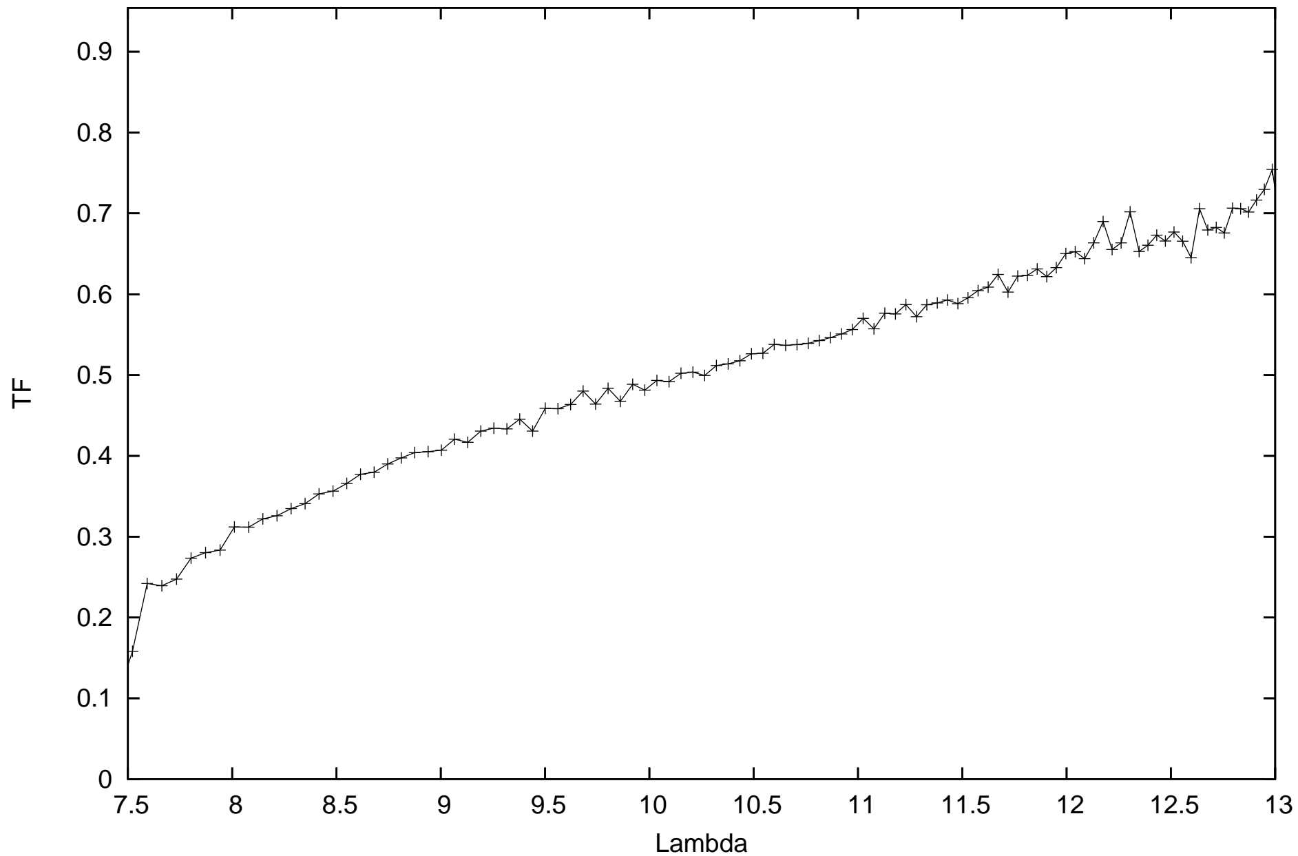
calHD133216_flux-1.76_diam11.15_r.MIDI.2011-02-11T08_31_39.000_H0G1
