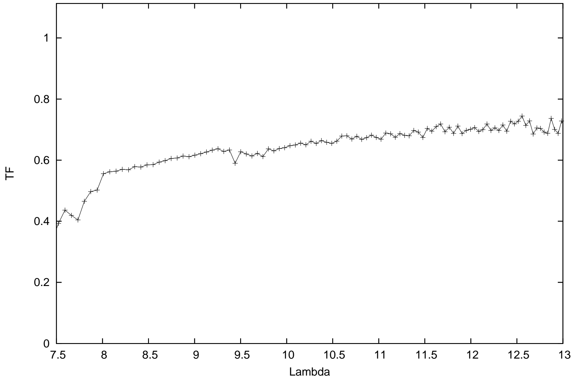
calHD142804_flux1.33_diam2.82_r.MIDI.2011-04-18T10_19_38.000_U2U4
