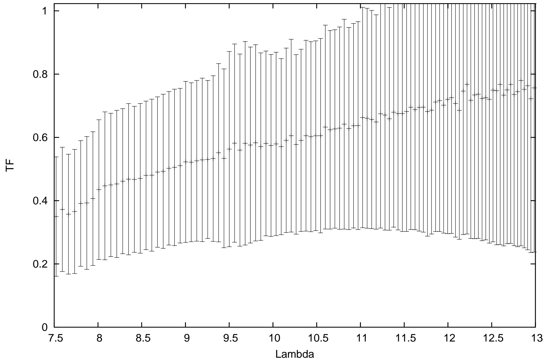
calHD149401_flux1.58_diam2.42_r.MIDI.2011-04-12T07_47_53.000_U2U3
