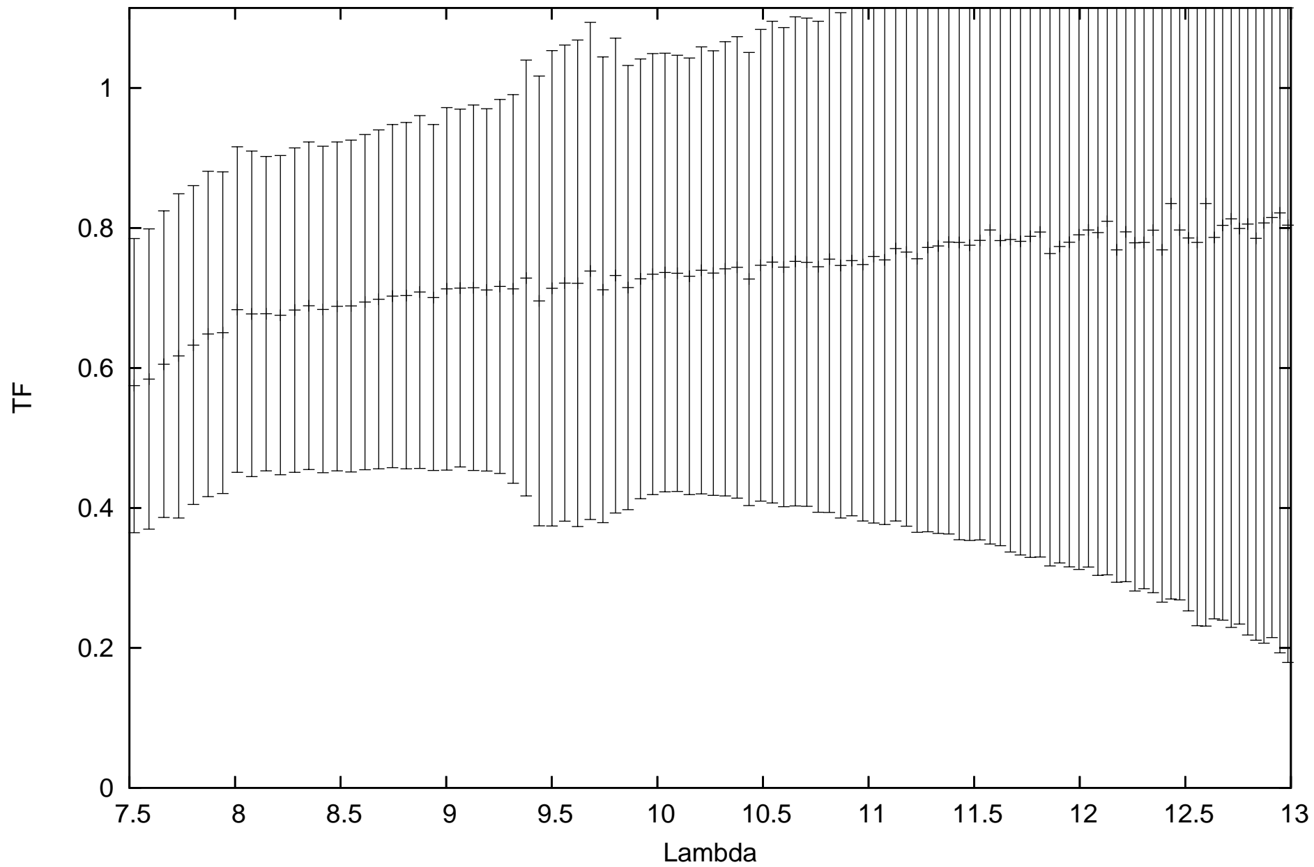
calHD149401_flux1.58_diam2.42_r.MIDI.2011-04-15T09_22_44.000_U2U3
