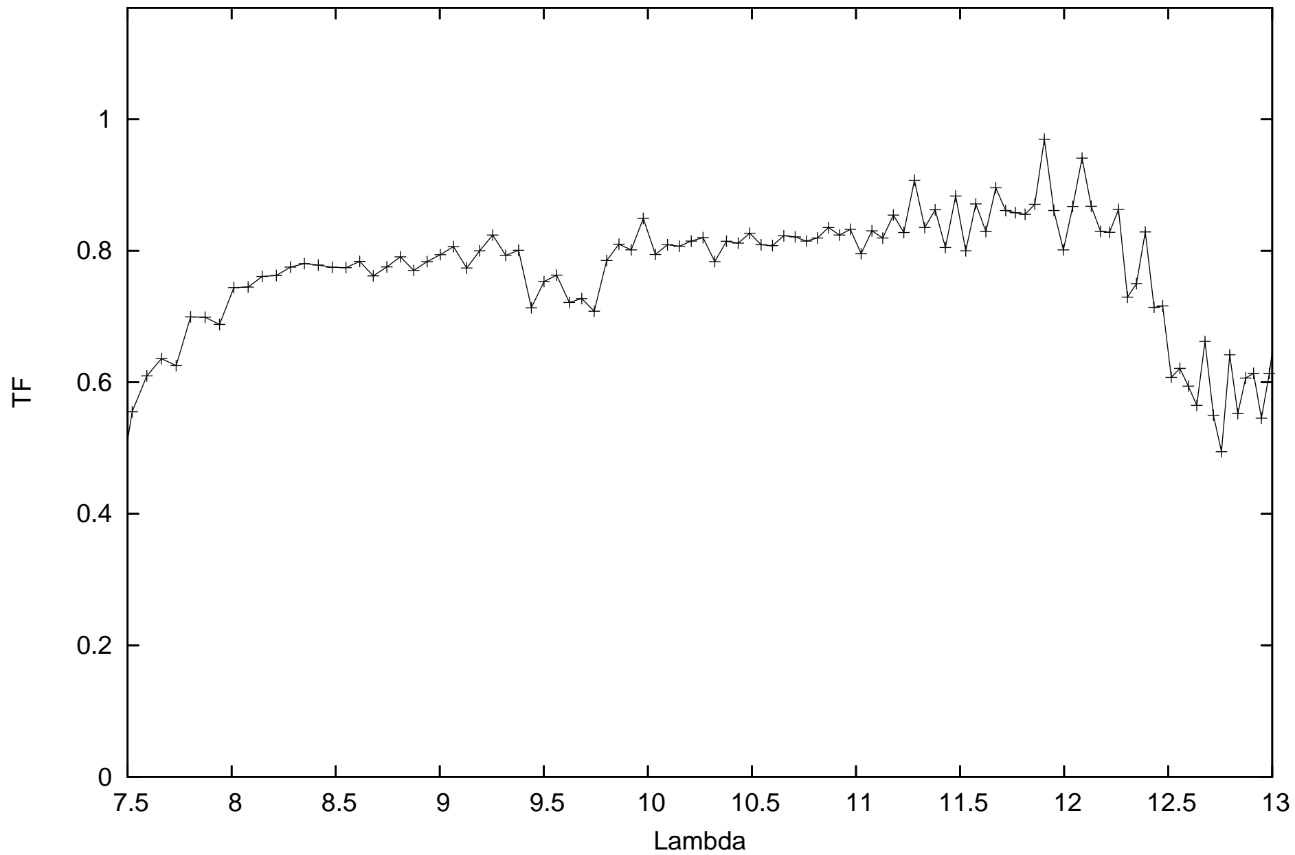
calHD152161_flux-0.26_diam6.12_r.MIDI.2011-07-27T00_59_40.000_G1A1
