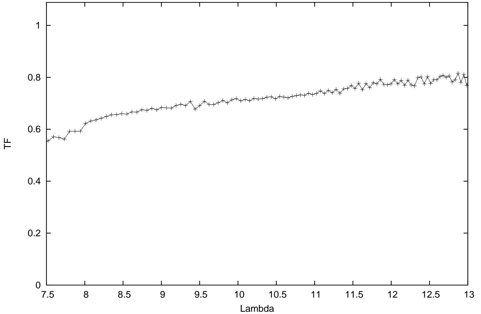
calHD157236_flux1.45_diam2.51_r.MIDI.2011-05-14T06_24_15.000_U3U4
