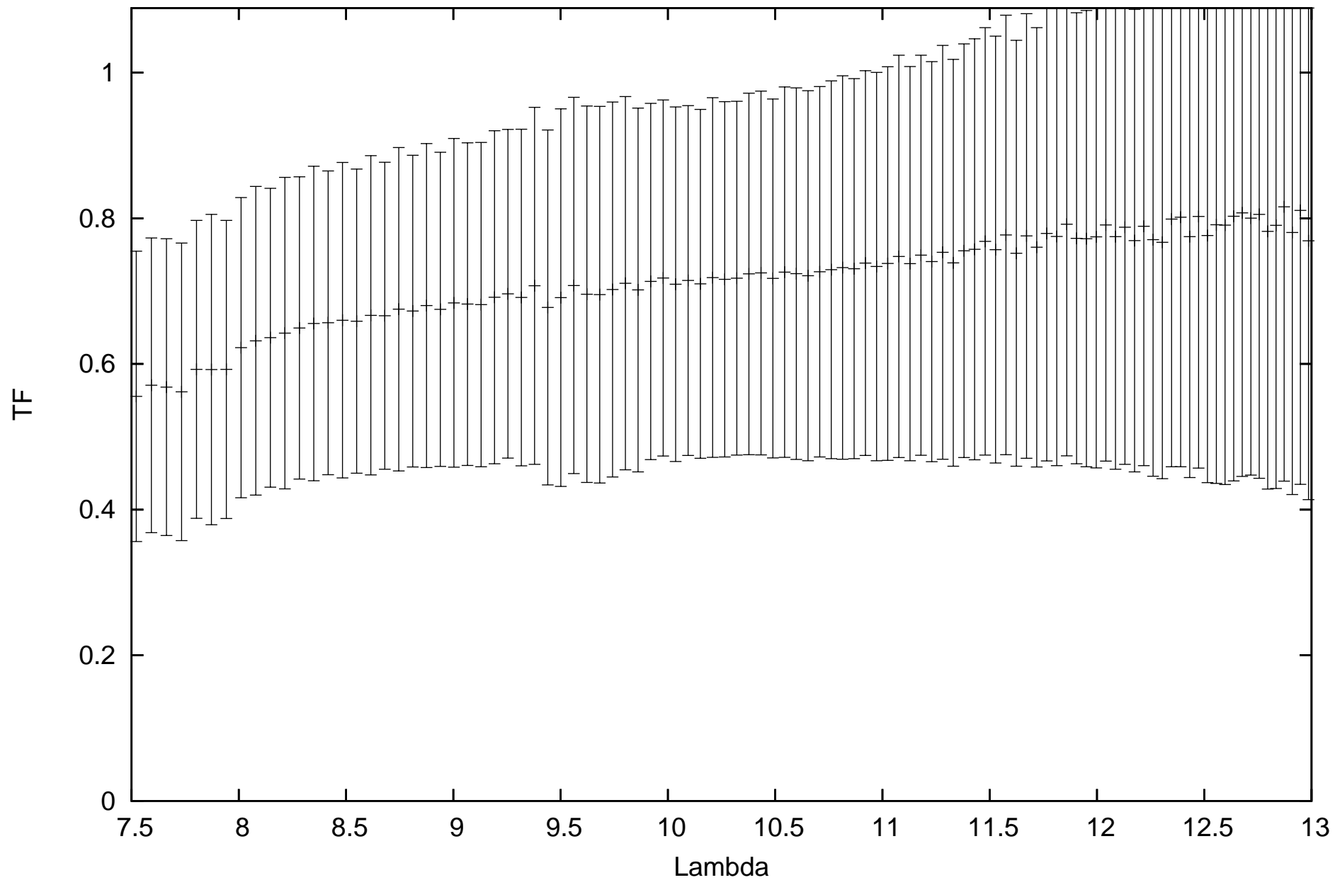
calHD157236_flux1.45_diam2.51_r.MIDI.2011-05-14T06_24_15.000_U3U4
