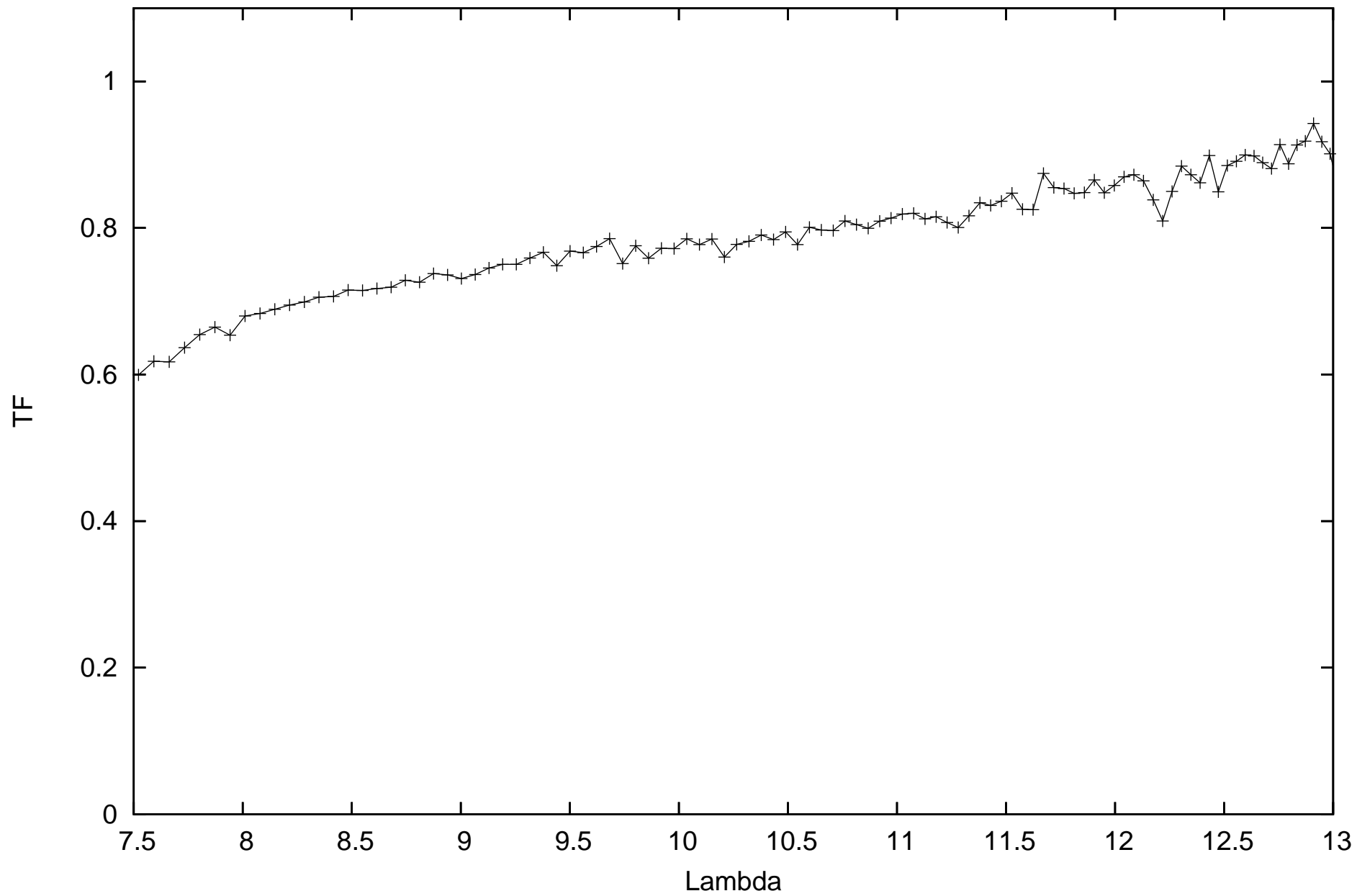
calHD159881_flux1.59_diam2.46_r.MIDI.2011-04-15T07_49_45.000_U2U3
