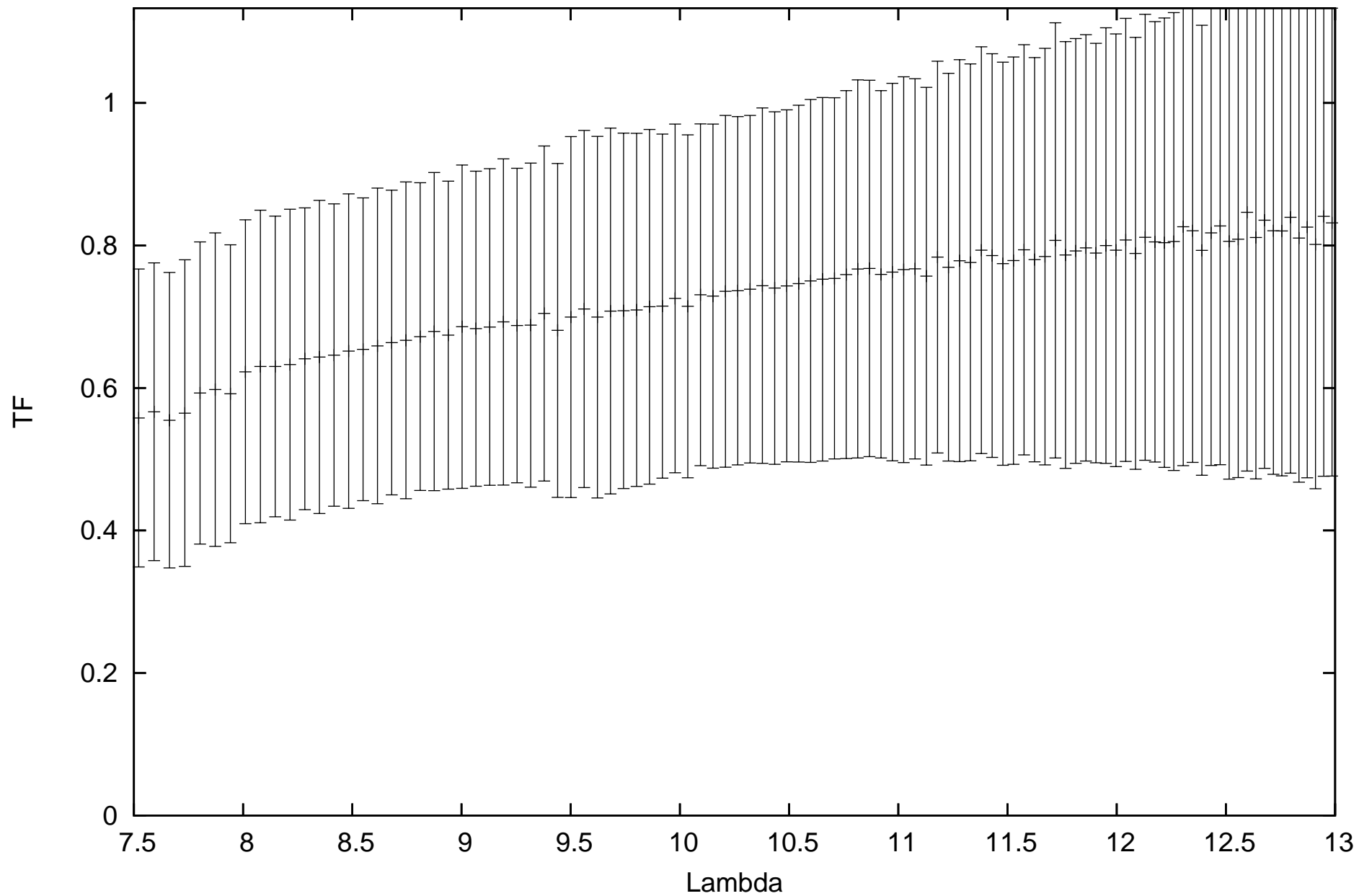
calHD159881_flux1.59_diam2.46_r.MIDI.2011-05-14T07_06_32.000_U3U4
