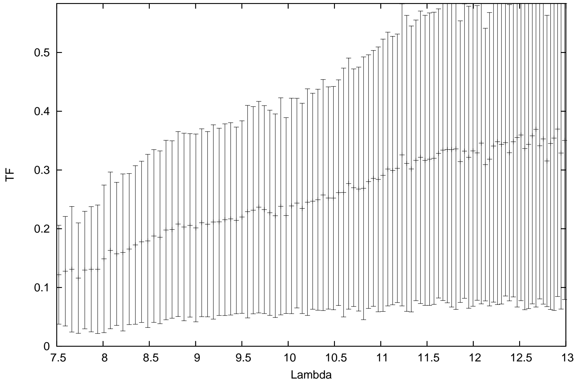
calHD167618_flux-1.82_diam11.66_r.MIDI.2011-06-07T08_37_51.000_D0C1
