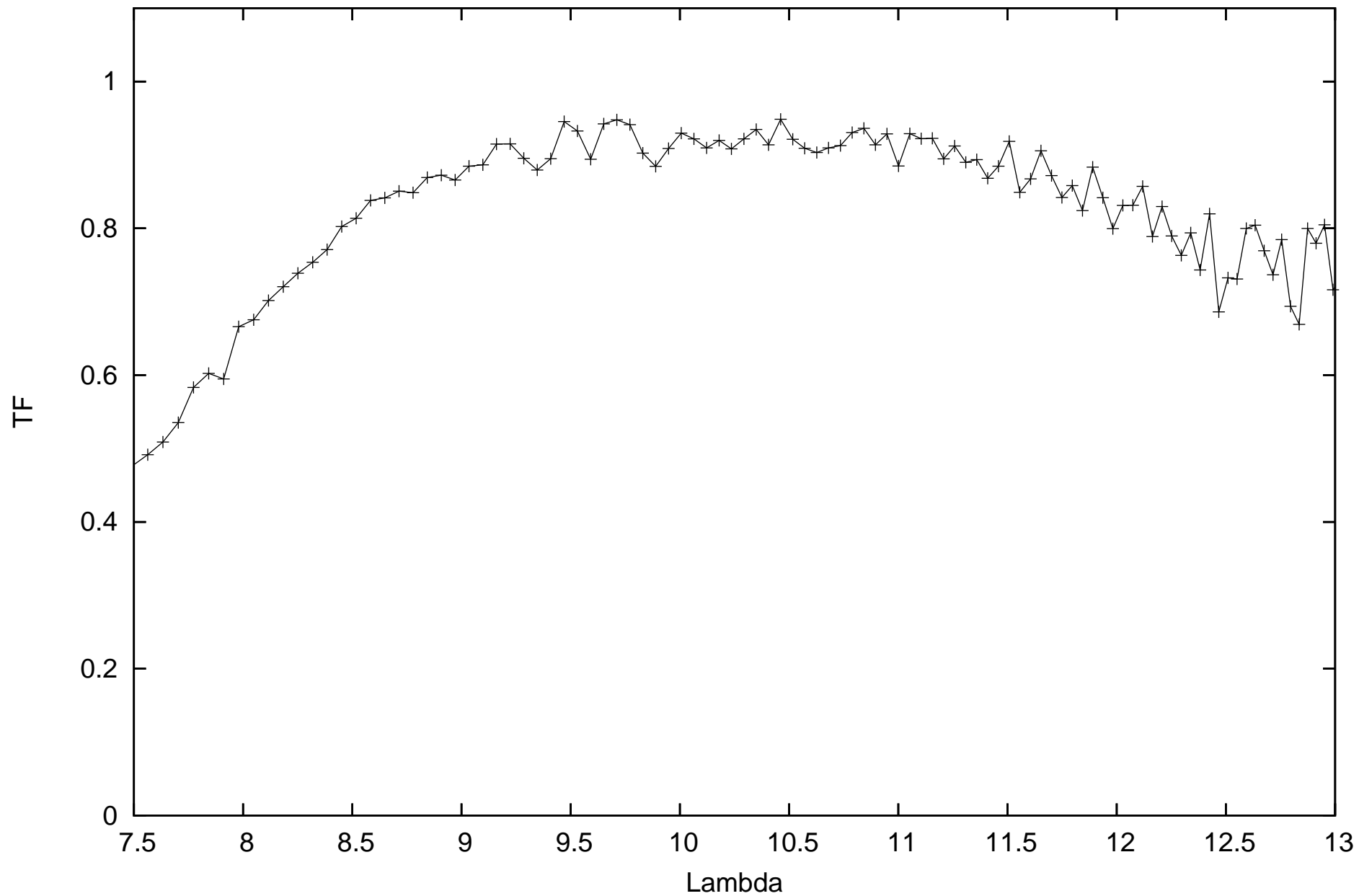
calHD167618_flux-1.82_diam11.66_r.MIDI.2011-06-12T07_02_43.015_B2A1
