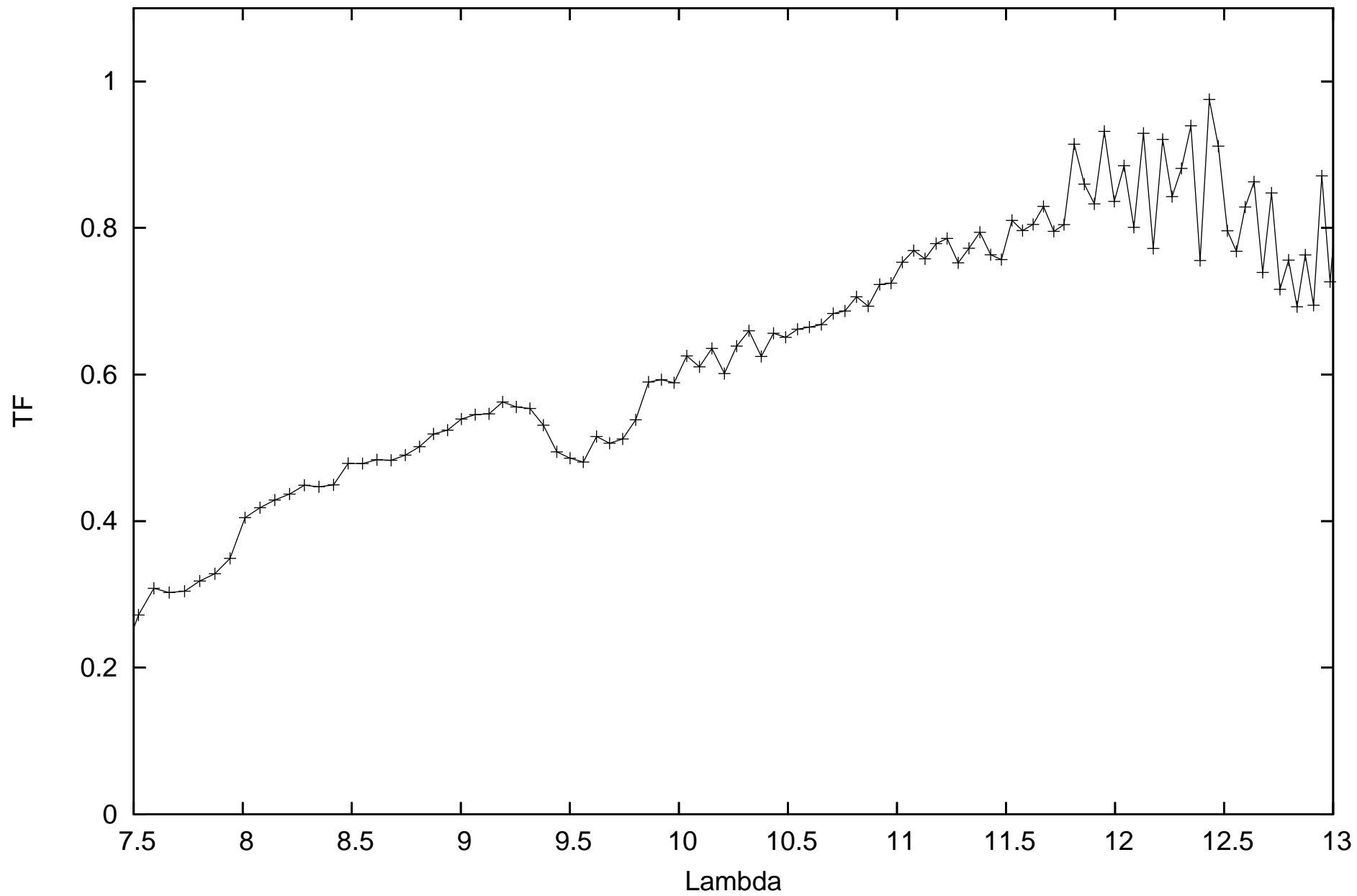
calHD167618_flux-1.82_diam11.66_r.MIDI.2011-07-02T06_07_49.000_D0G1
