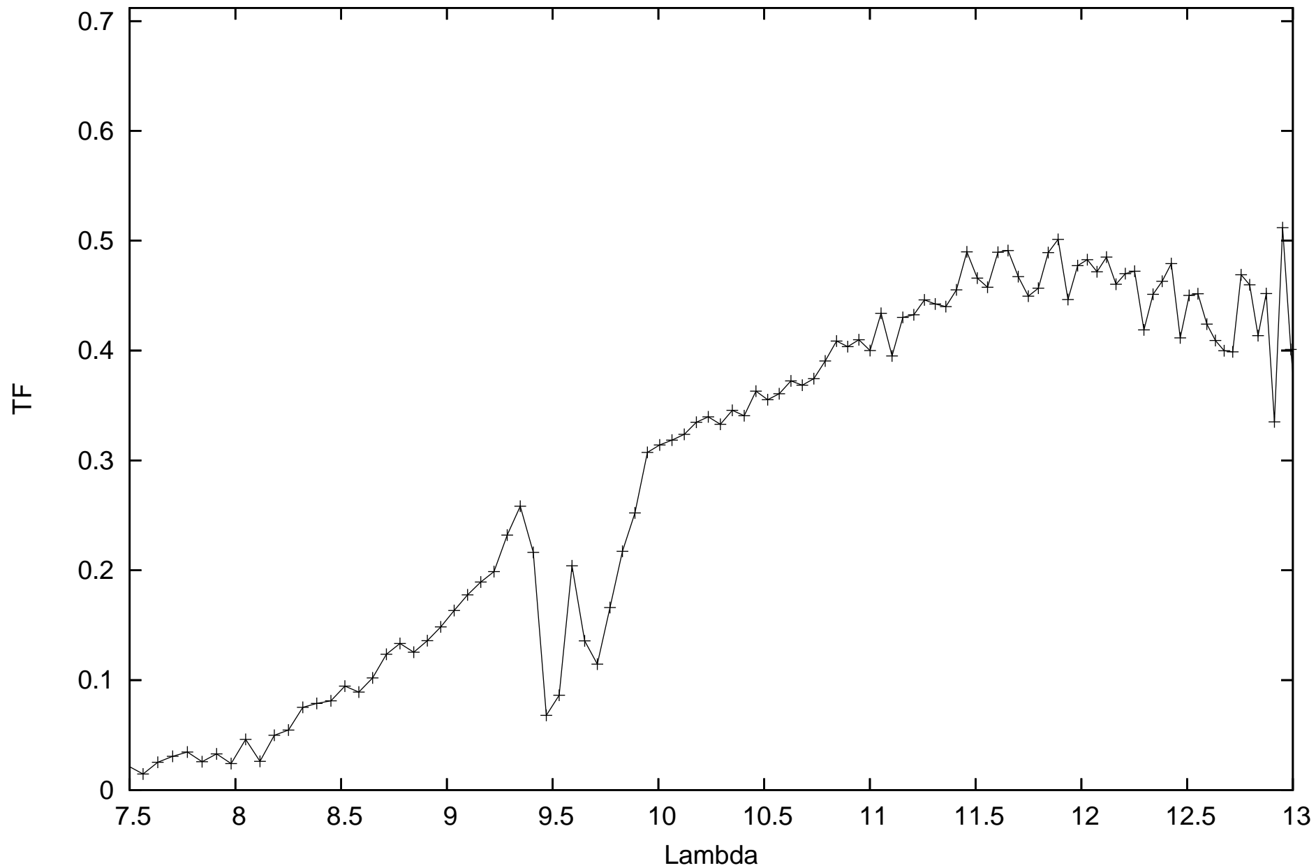
calHD167618_flux-1.82_diam11.66_r.MIDI.2011-10-06T00_48_01.113_K0A1
