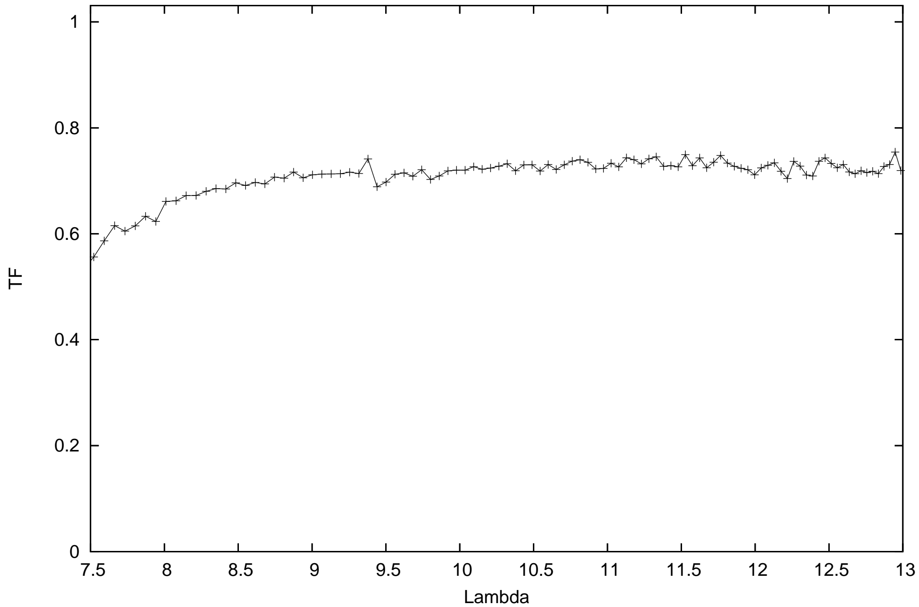
calHD167618_flux-1.82_diam11.66_r.MIDI.2011-10-22T23_54_44.000_C1A1
