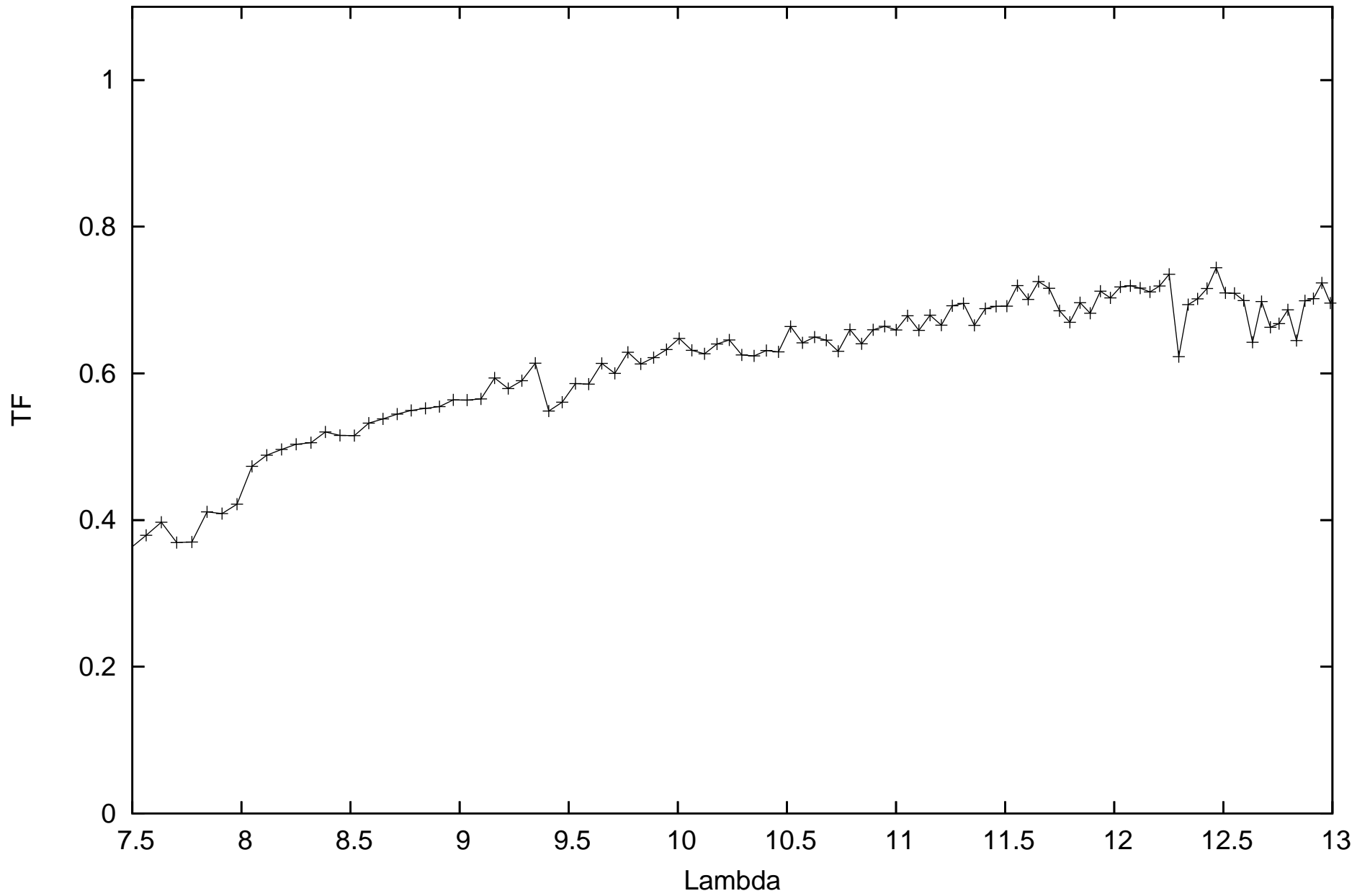
calHD167618_flux-1.82_diam11.66_r.MIDI.2011-11-04T23_51_17.135_H0I1
