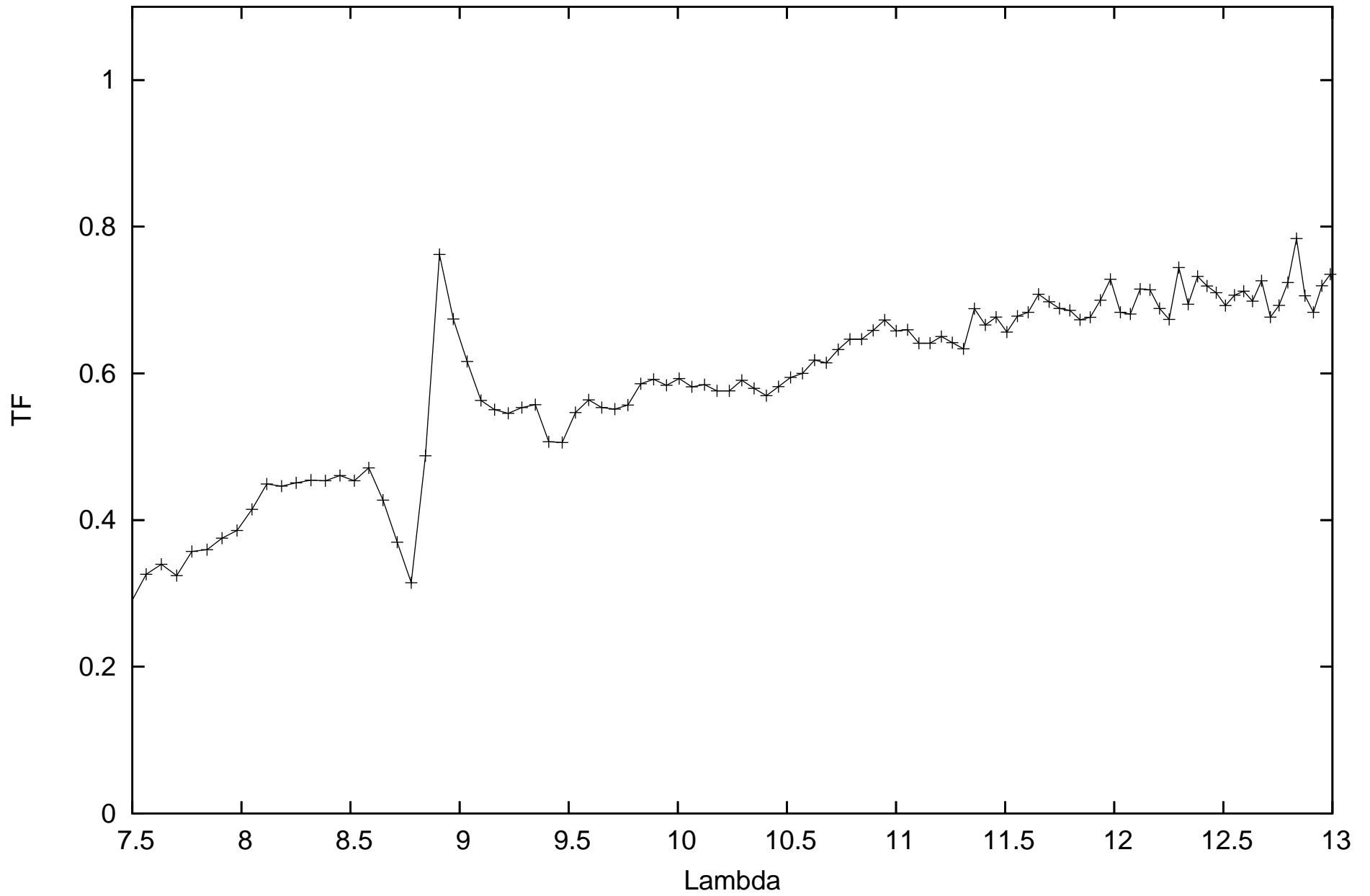
calHD167618_flux-1.82_diam11.66_r.MIDI.2011-11-05T23_48_45.969_H011
