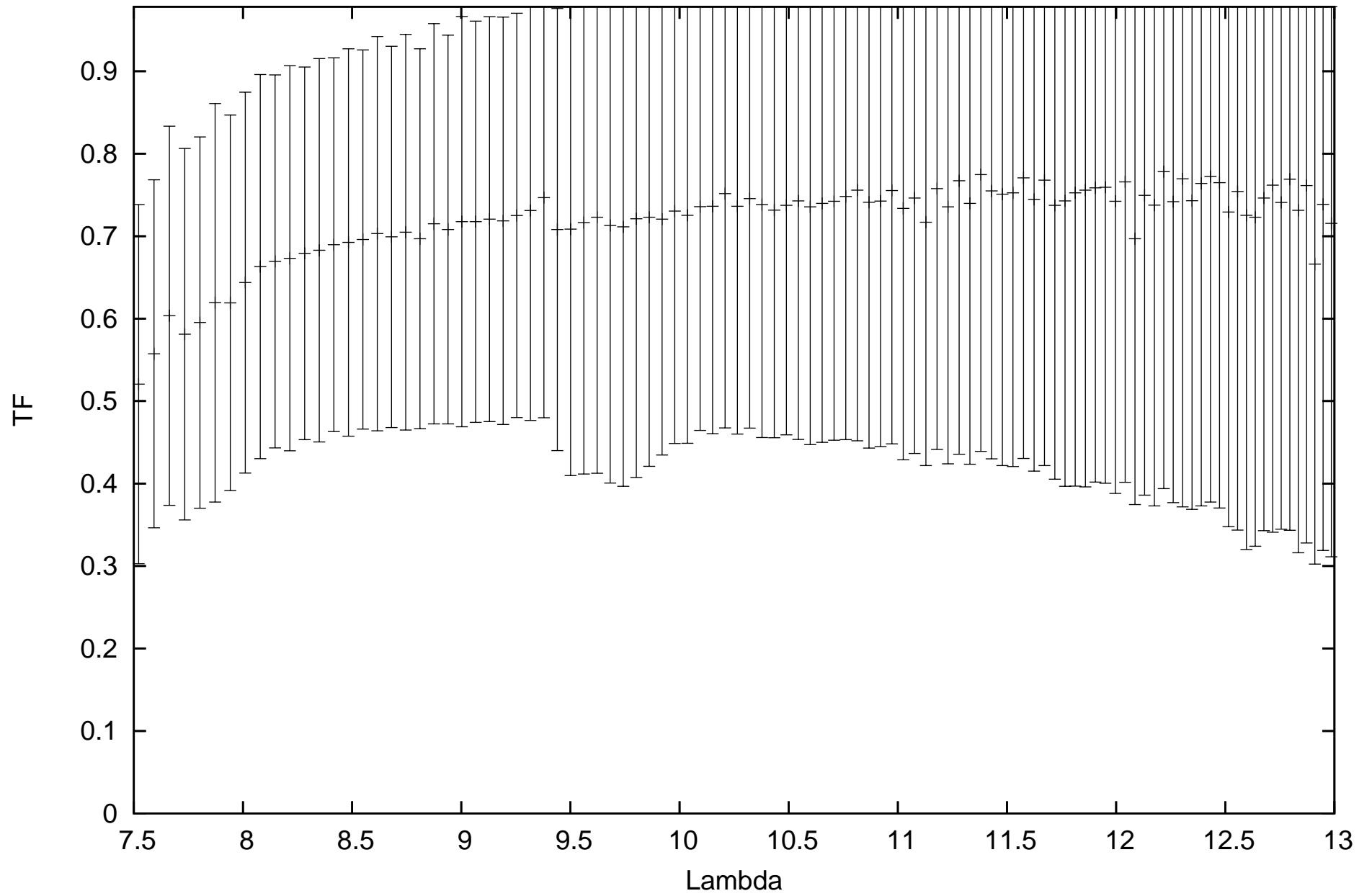
calHD18700_flux1.69_diam2.29_r.MIDI.2011-12-11T00_21_59.000_U2U3
