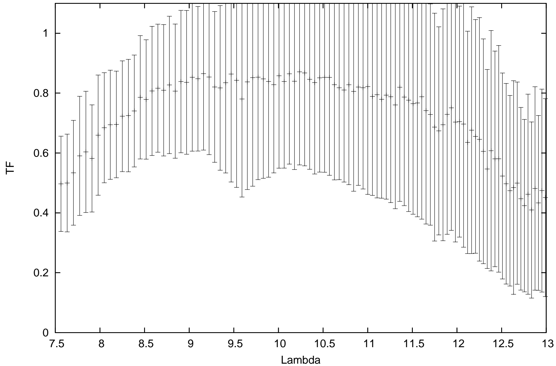
calHD206778_flux-1.04_diam7.59_r.MIDI.2011-06-11T09_43_40.946_C1A1
