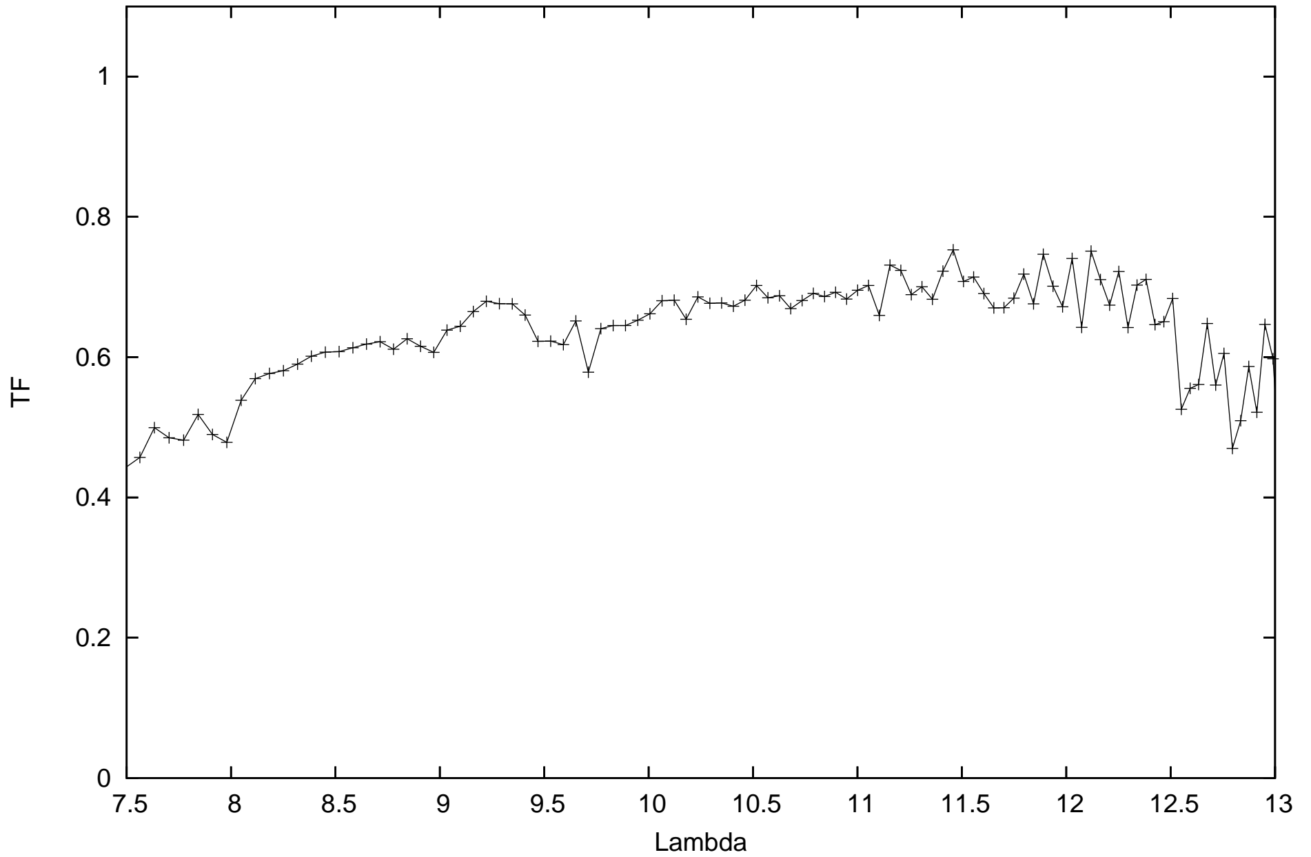
calHD20720_flux-1.53_diam10.14_r.MIDI.2011-10-24T06_16_04.970_D0A1
