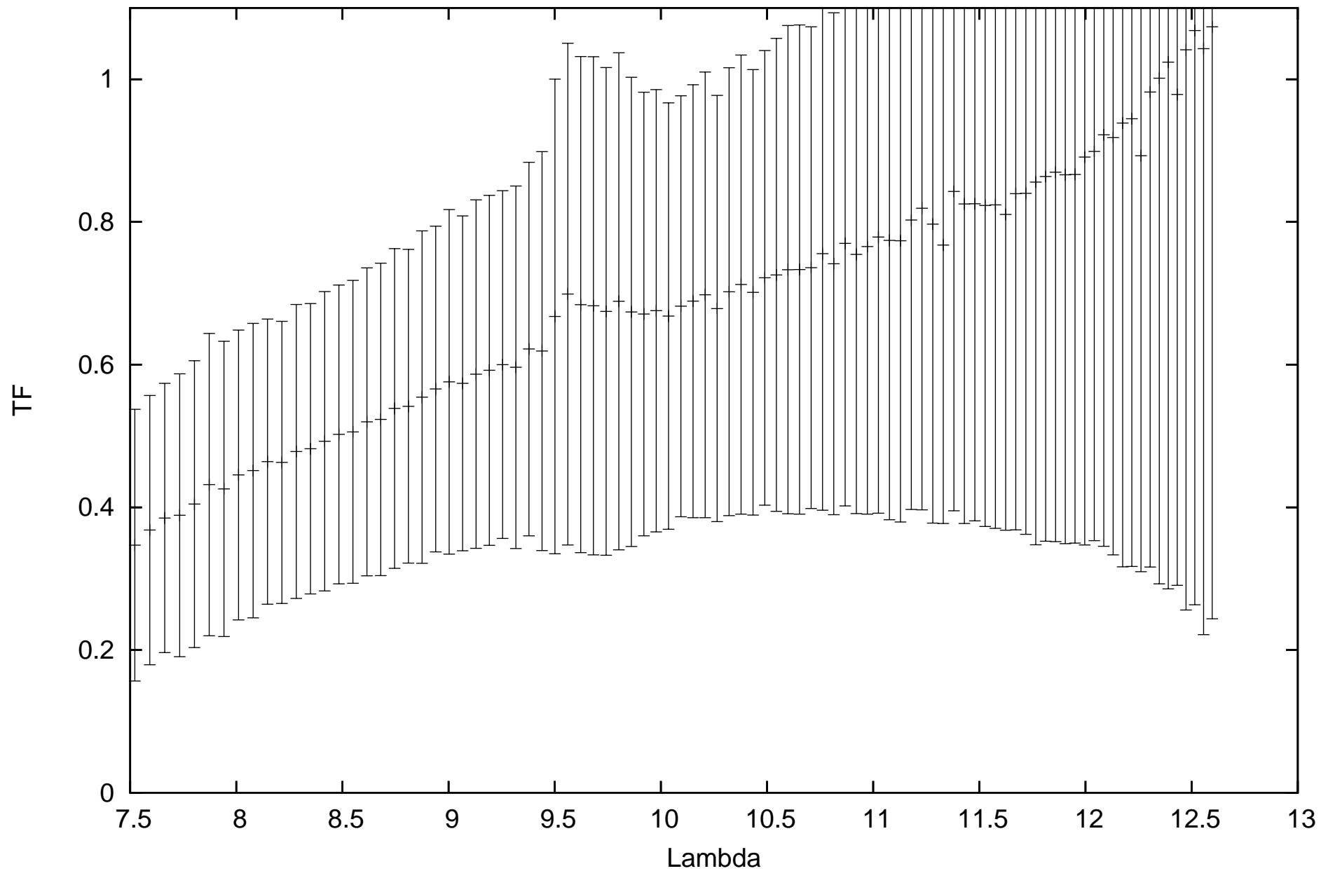
calHD20720_flux-1.53_diam10.14_r.MIDI.2011-11-16T02_47_19.000_K0G1
