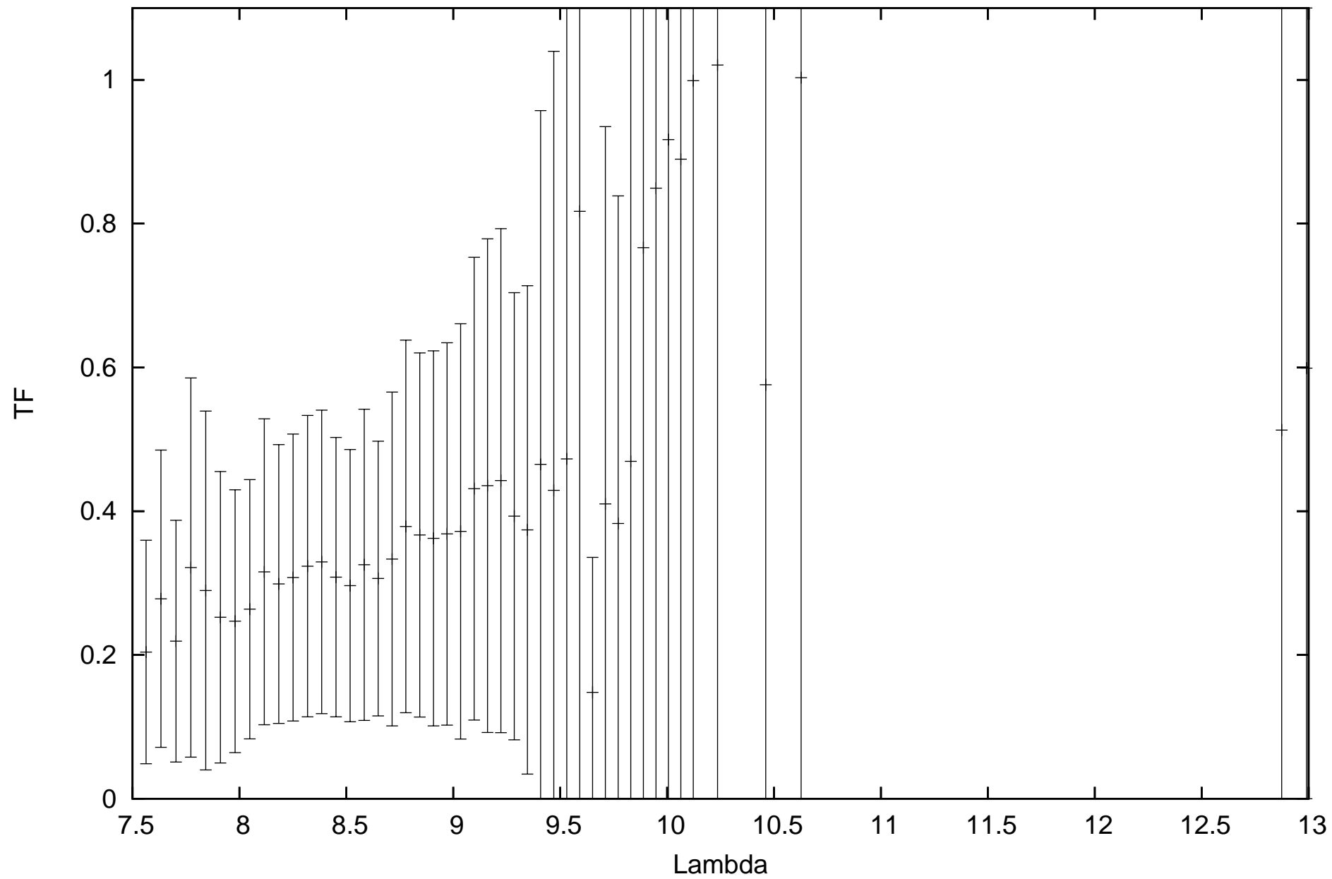
calHD224935_flux-0.85_diam7.24_r.MIDI.2011-08-11T09_18_47.015_B2A1
