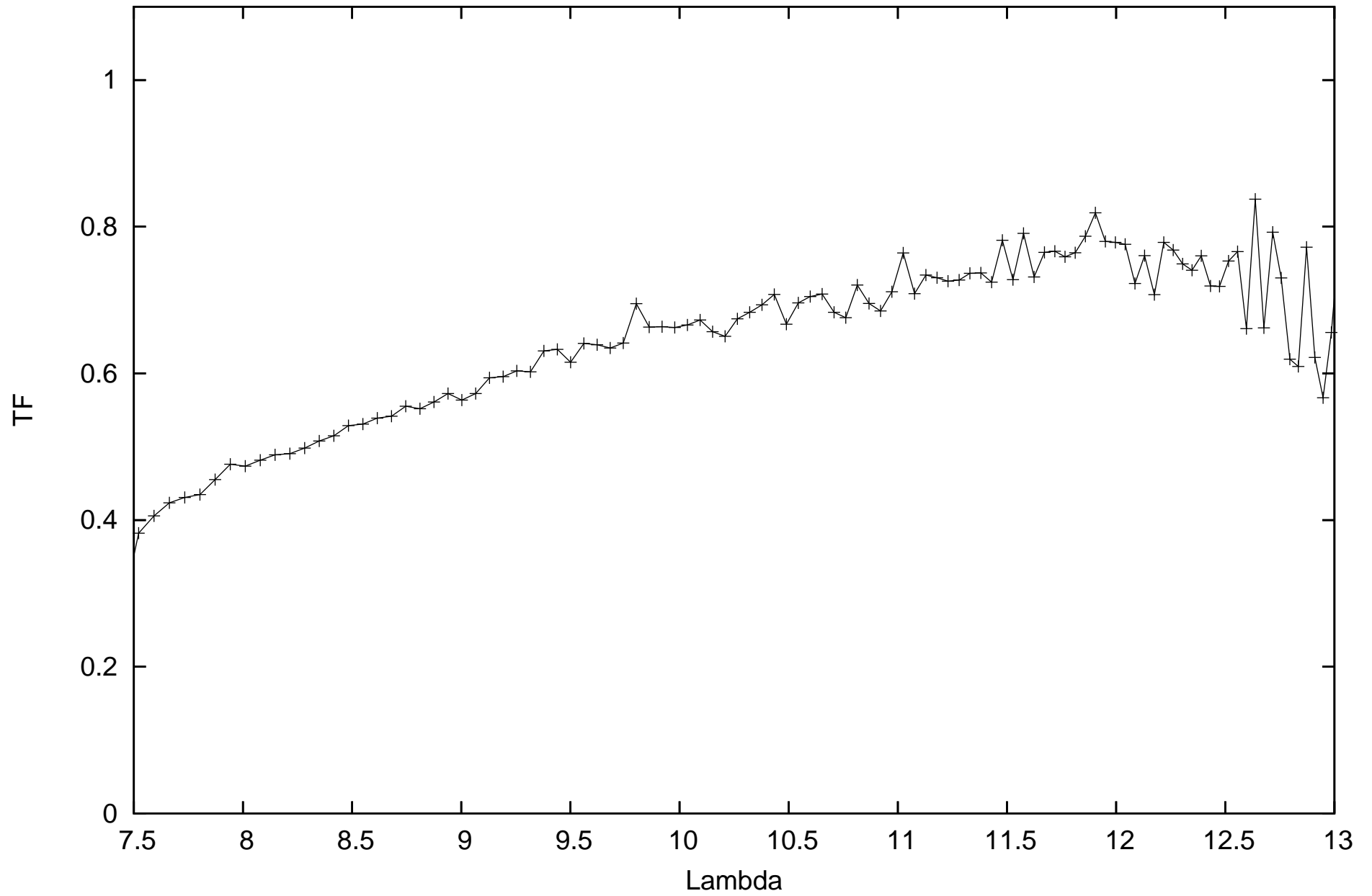
calHD224935_flux-0.85_diam7.24_r.MIDI.2011-10-05T06_36_49.000_J3A1
