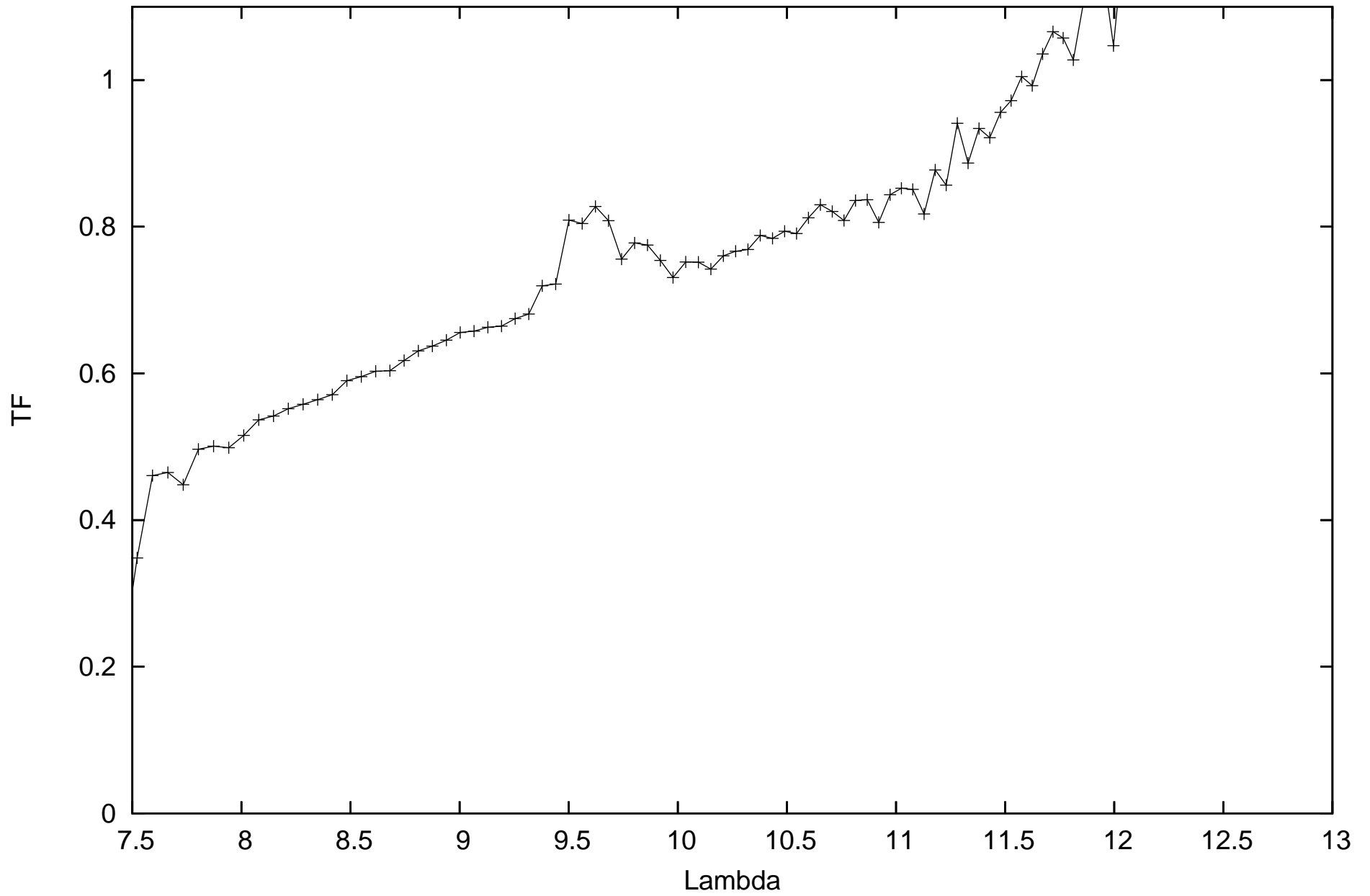
calHD224935_flux-0.85_diam7.24_r.MIDI.2011-10-31T00_42_44.000_K0G1
