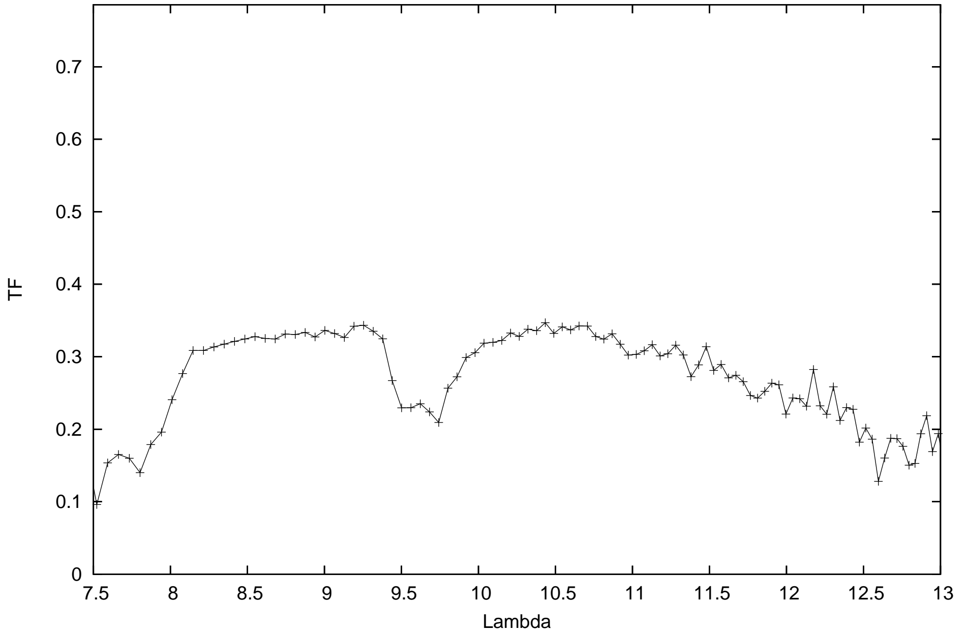
calHD224935_flux-0.85_diam7.24_r.MIDI.2011-11-01T01_44_54.000_K0A1
