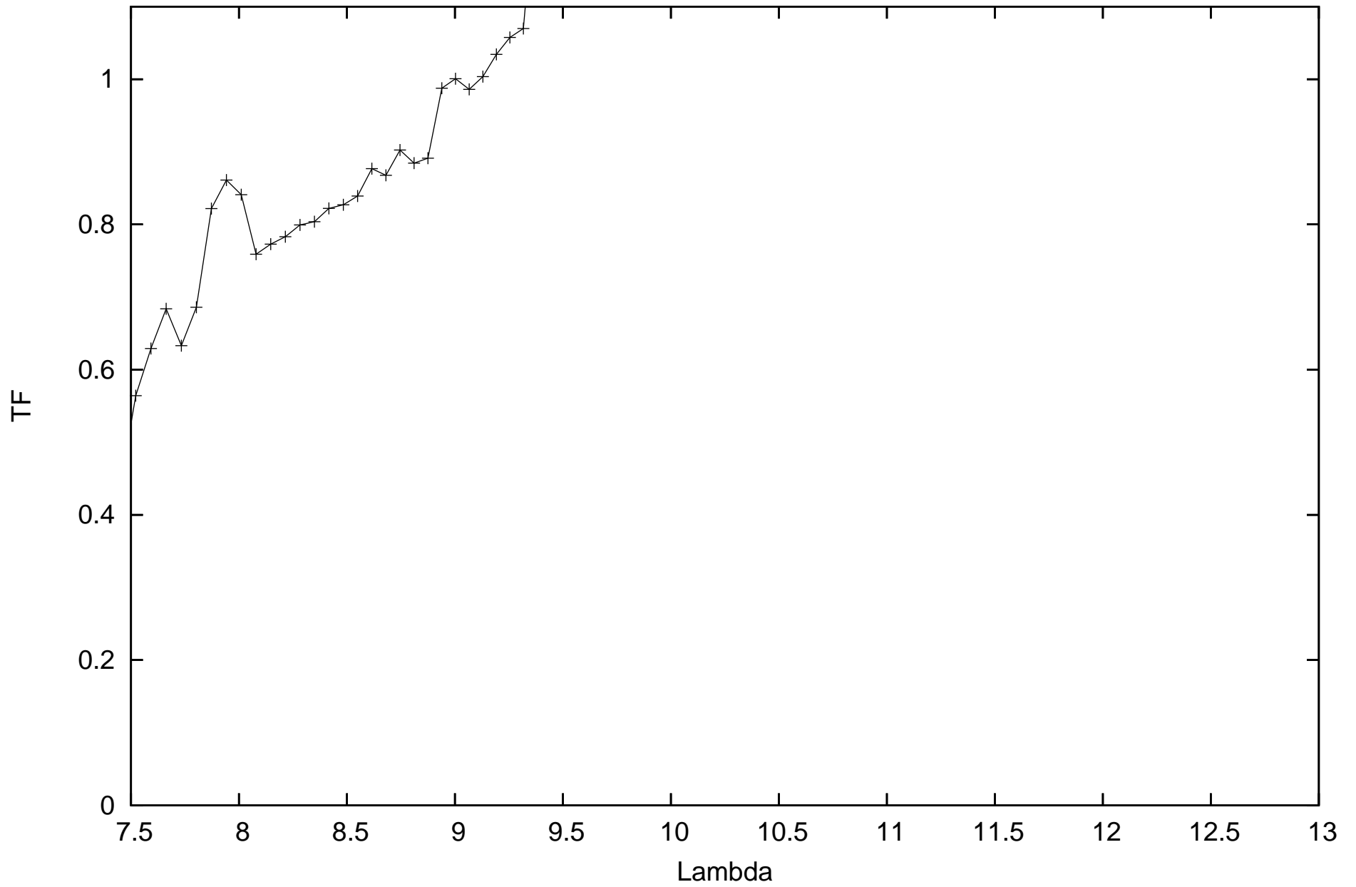
calHD33684_flux0.03_diam5.07_r.MIDI.2011-10-05T08_06_41.000_J3A1
