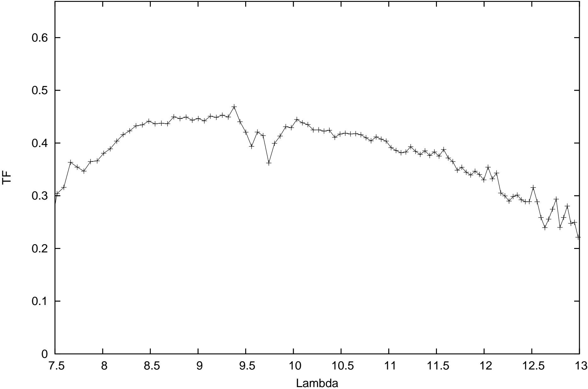
calHD48915_flux-1.39_diam6.09_r.MIDI.2011-10-02T09_24_01.000_J3G1
