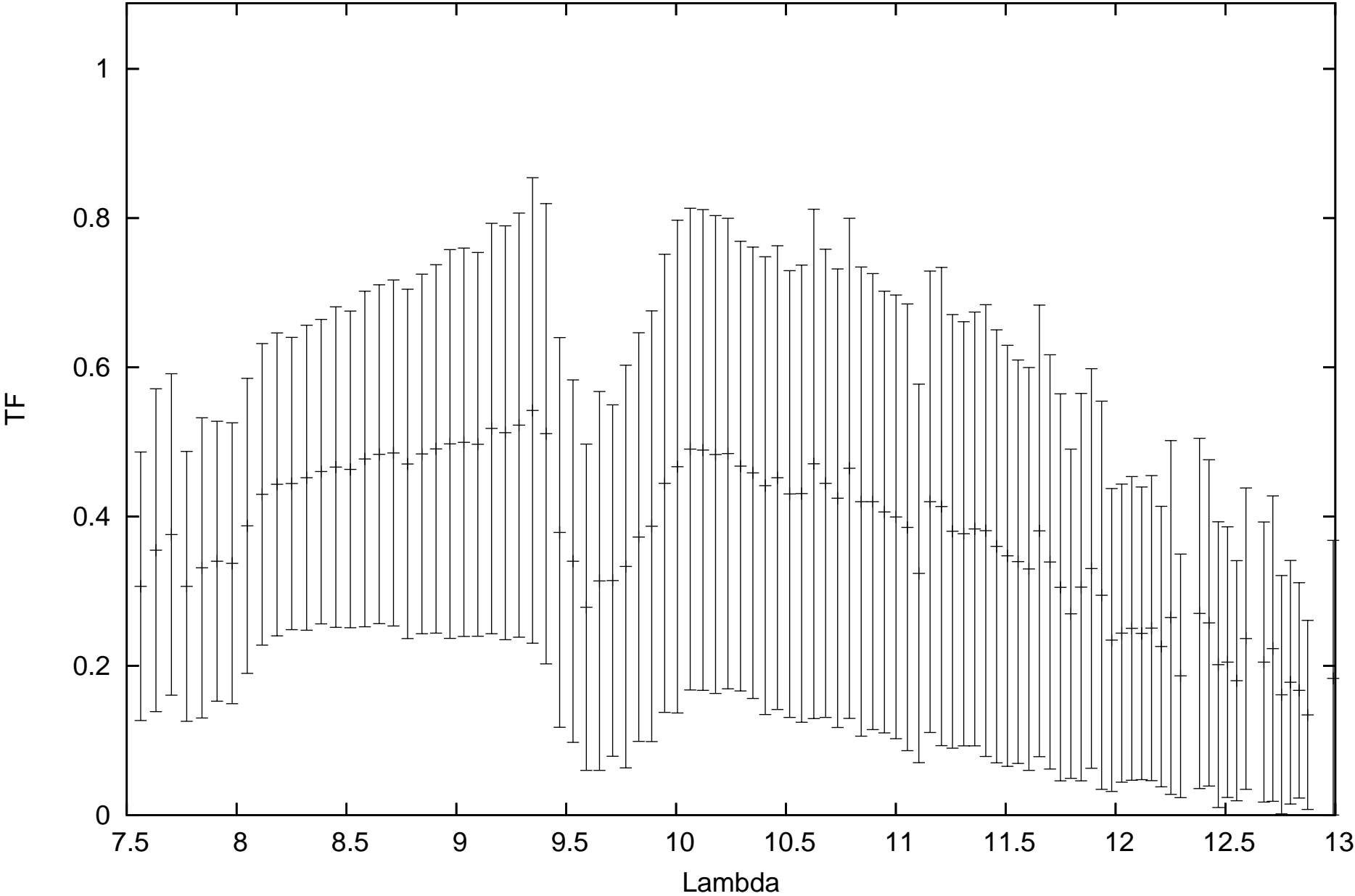
calHD48915_flux-1.39_diam6.09_r.MIDI.2011-10-02T09_32_36.112_J3G1
