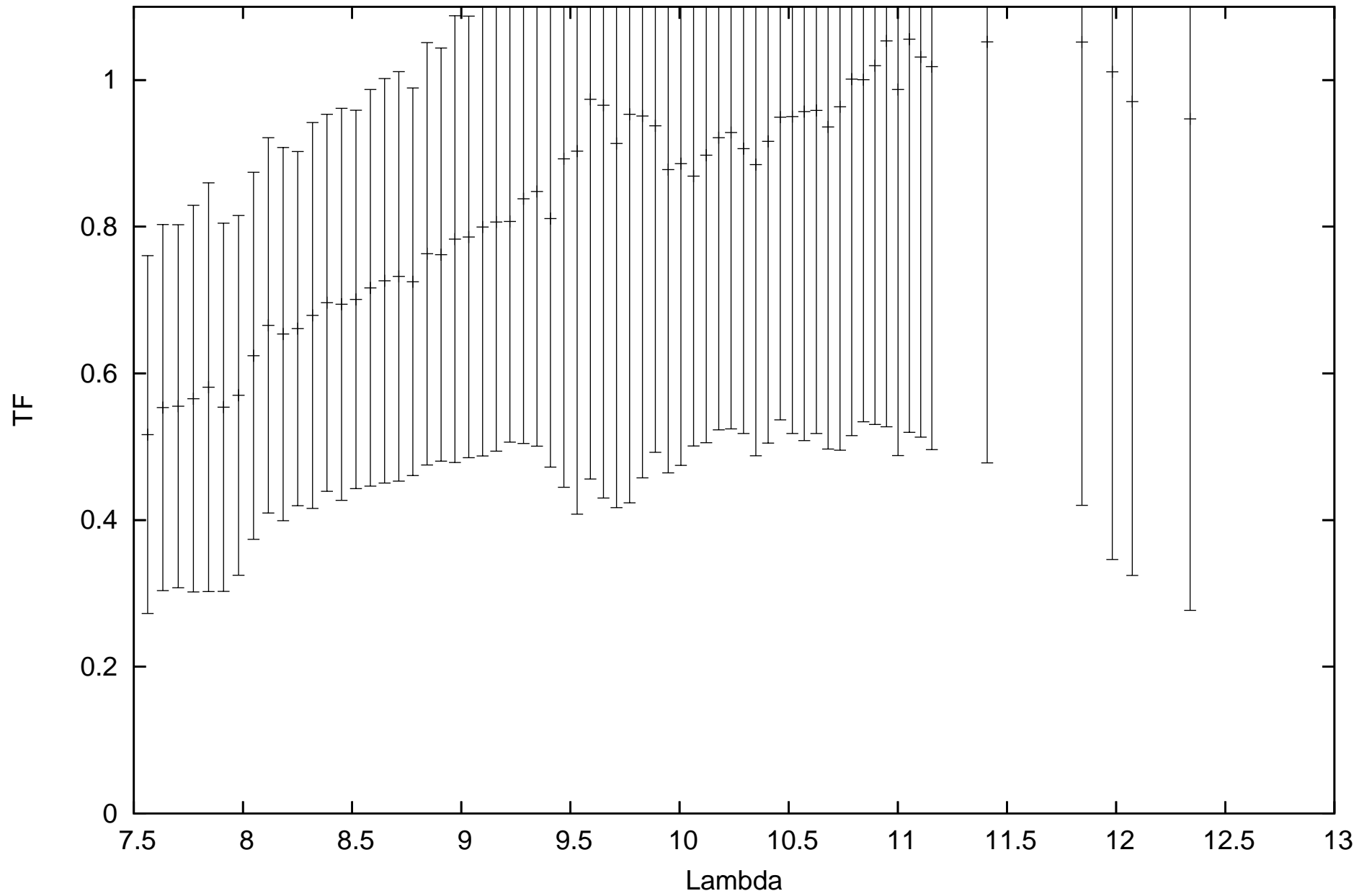
calHD48915_flux-1.39_diam6.09_r.MIDI.2011-10-24T06_54_28.135_D0A1
