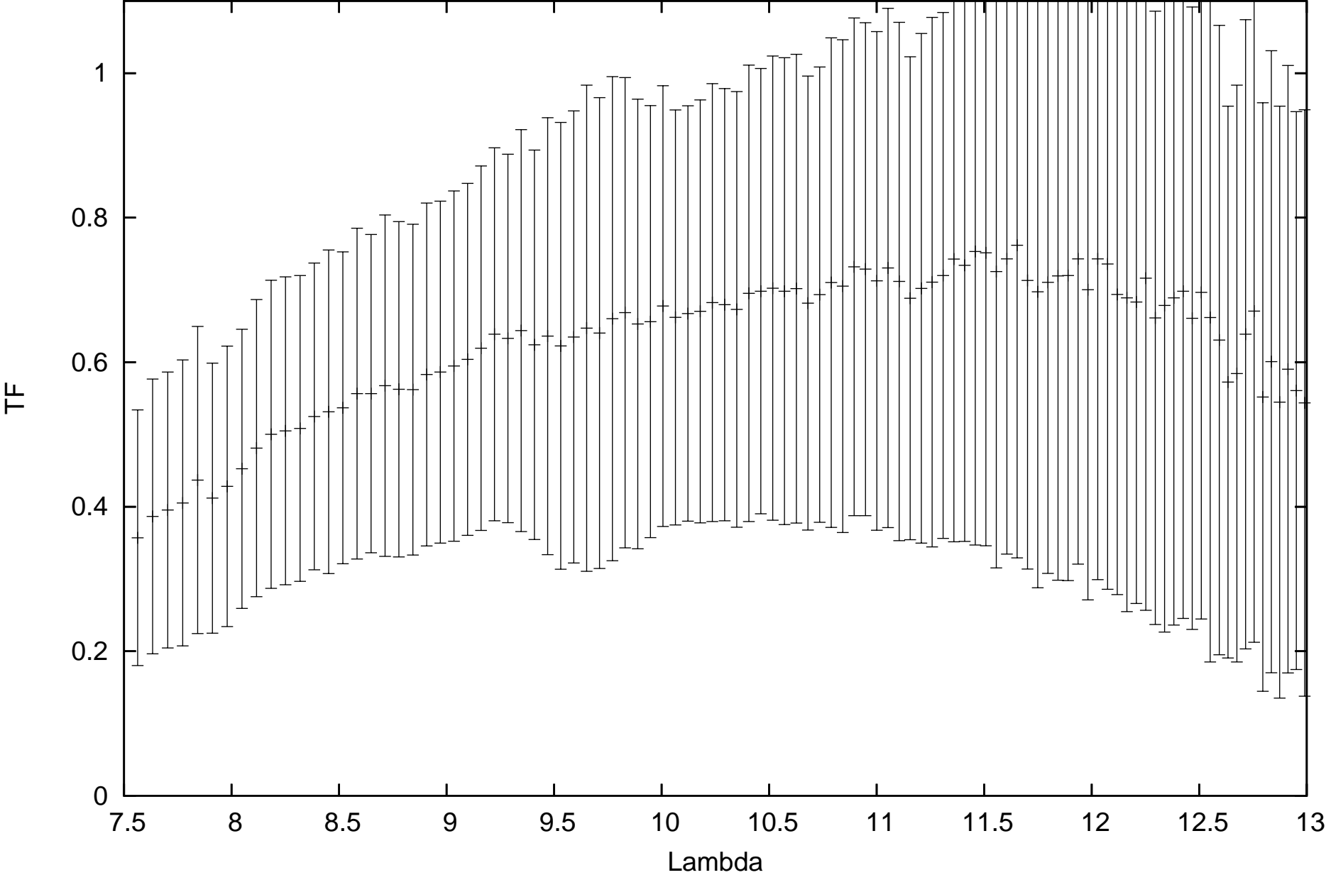
calHD48915_flux-1.39_diam6.09_r.MIDI.2011-12-04T05_28_47.112_G1J3
