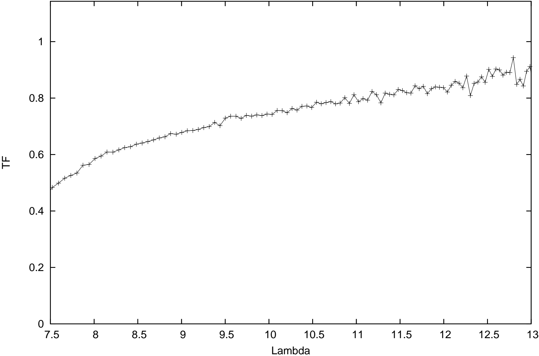
calHD48915_flux-1.39_diam6.09_r.MIDI.2011-12-04T05_59_36.000_J3G1
