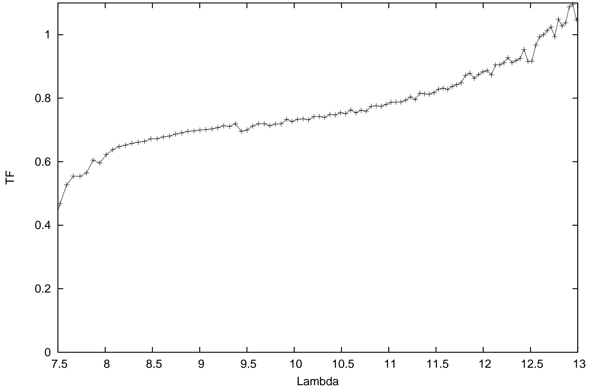
calHD63700_flux0.76_diam3.18_r.MIDI.2011-12-13T08_13_07.000_U3U4
