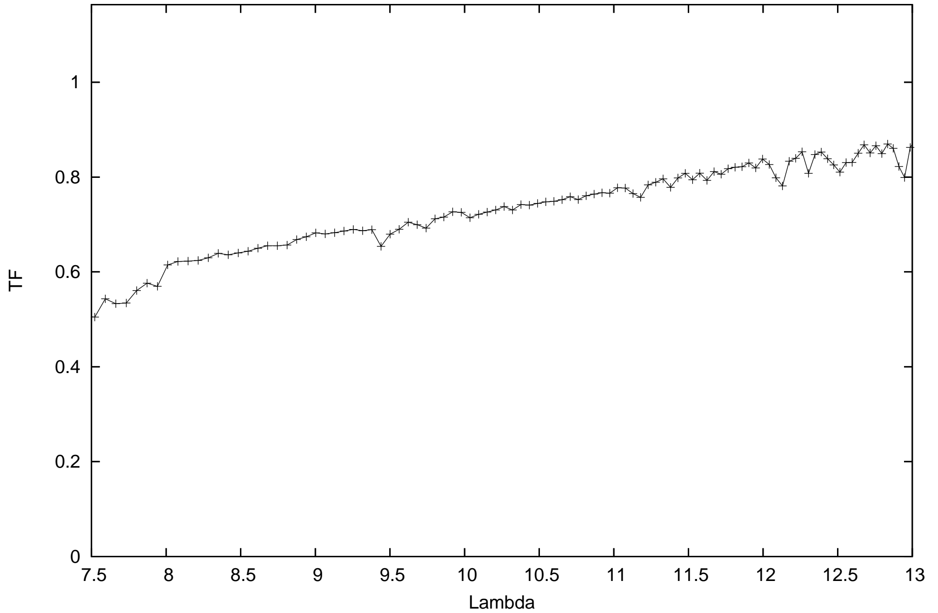
calHD63700_flux0.76_diam3.18_r.MIDI.2011-12-14T04_00_09.000_U2U3
