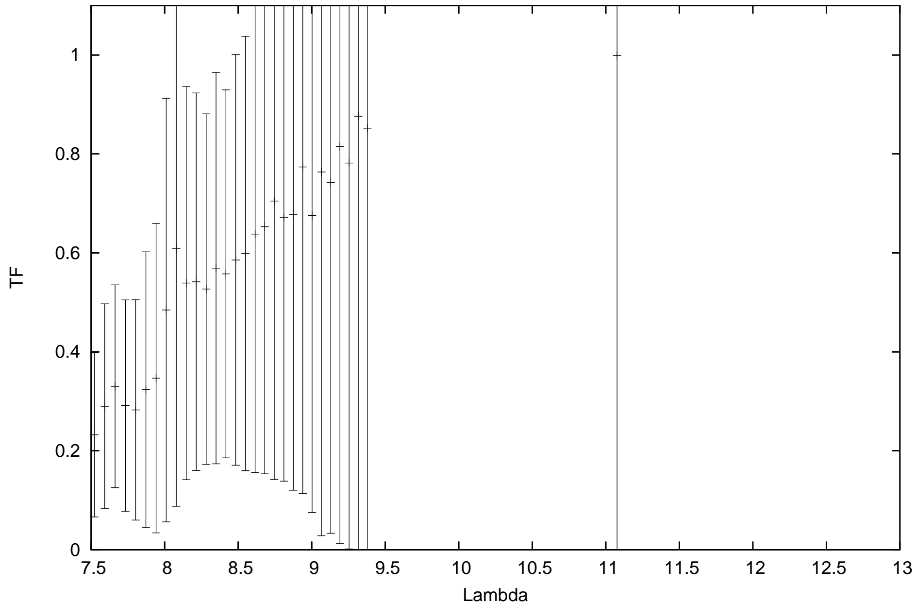
calHD68553_flux0.59_diam3.8_r.MIDI.2011-10-04T08_14_27.000_J3K0
