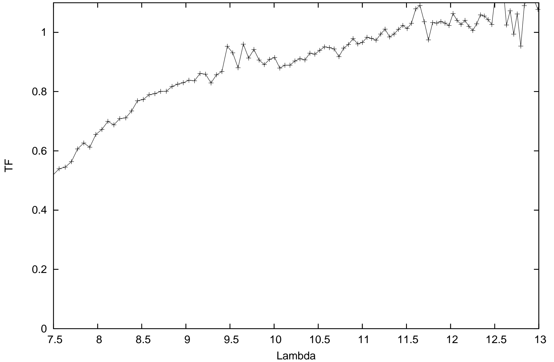
calHD81797_flux-1.49_diam9.14_r.MIDI.2010-12-08T08_24_12.015_D0H0
