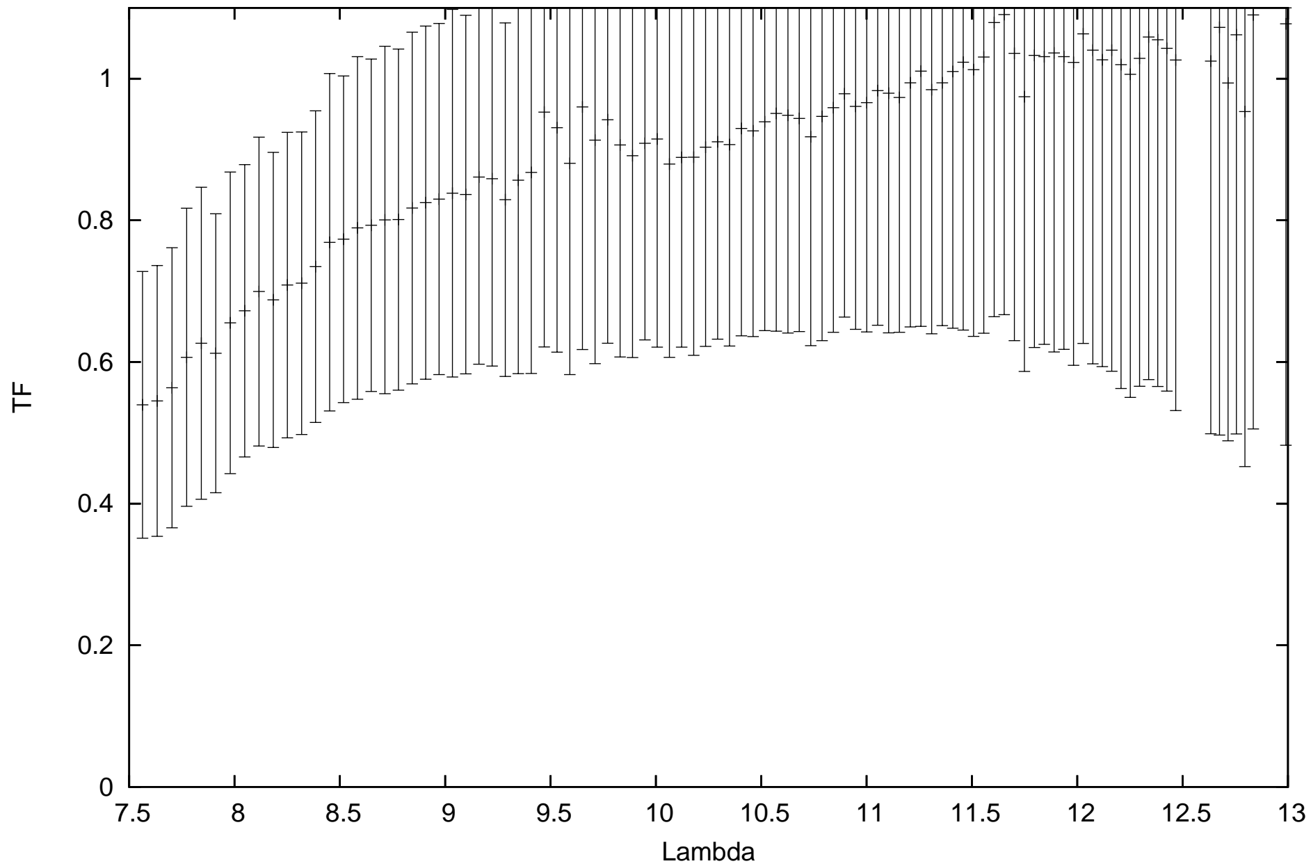
calHD81797_flux-1.49_diam9.14_r.MIDI.2010-12-08T08_24_12.015_D0H0
