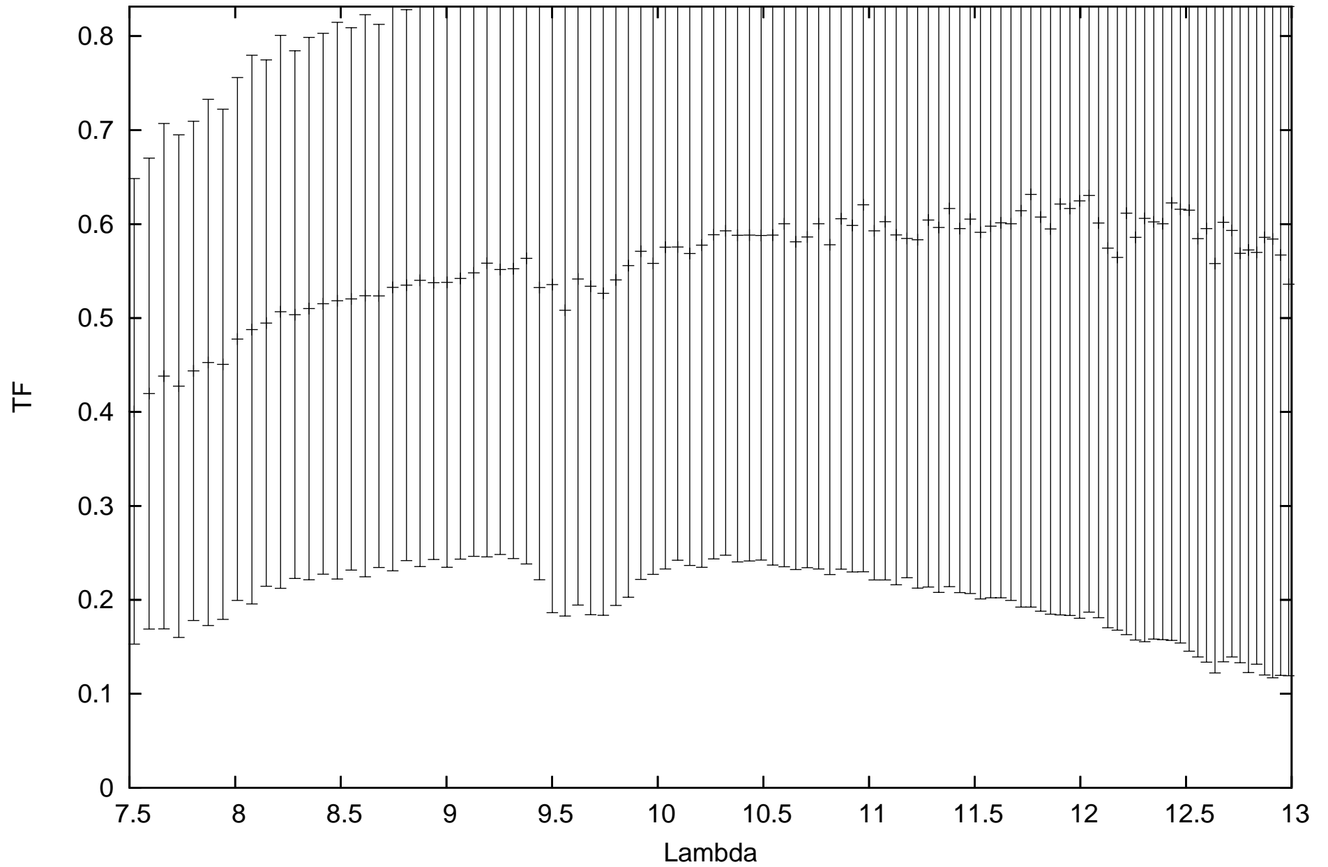
calHIP108699_flux2.12454_diam1.854582_r.MIDI.2011-10-10T00_51_22.000_U1U2
