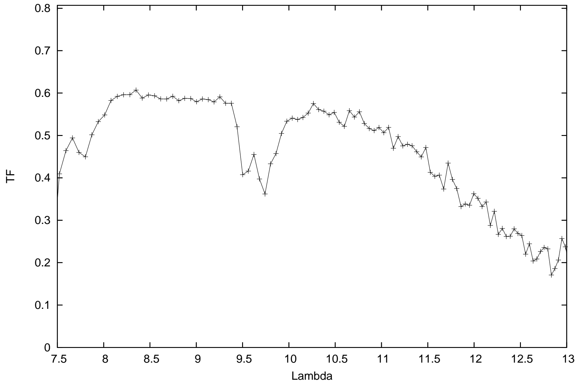
calHIP1170_flux-0.10766_diam5.17_r.MIDI.2011-10-30T03_41_42.000_G1A1
