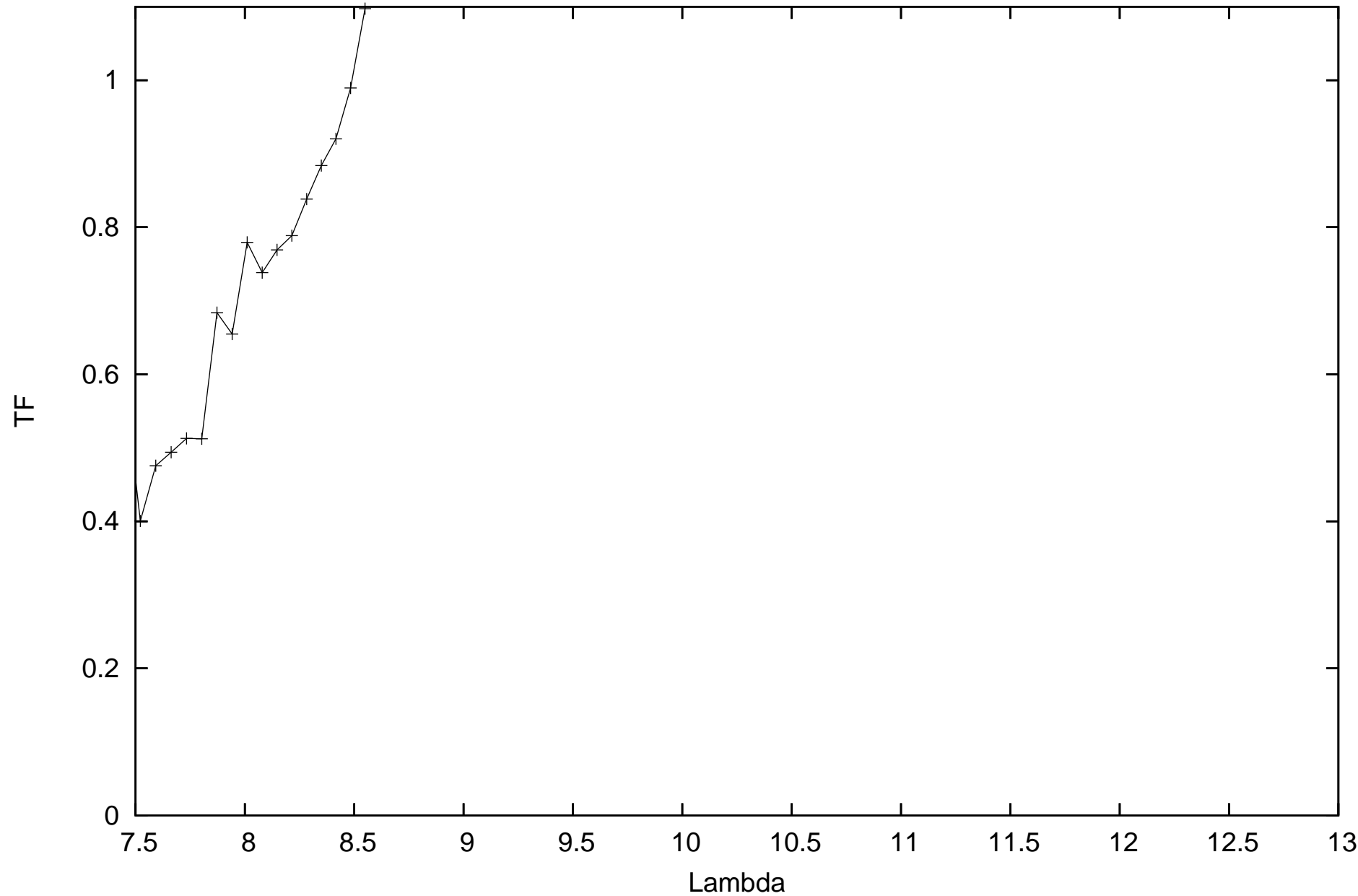
calHIP1170_flux-0.10766_diam5.17_r.MIDI.2011-10-31T01_09_52.000_K0G1
