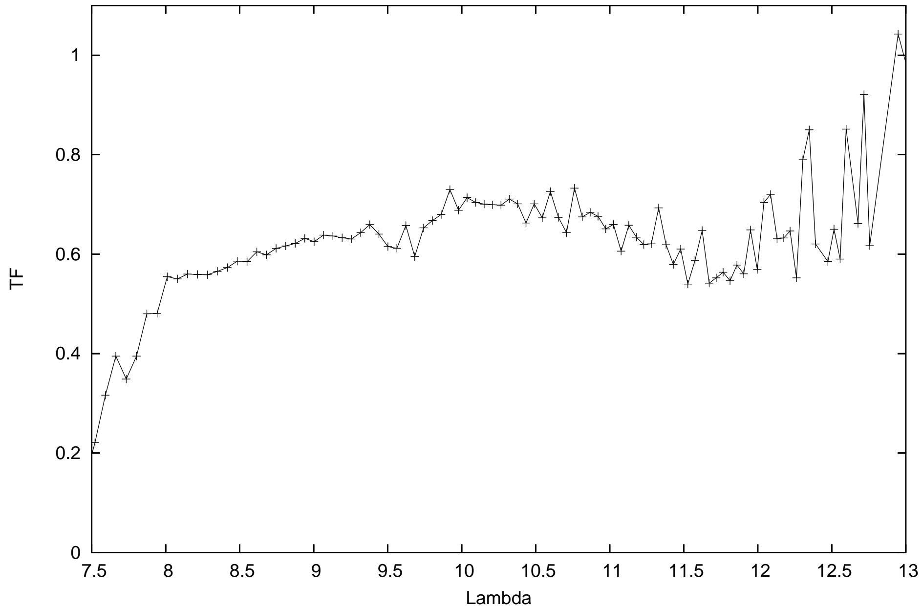
calHIP1170_flux-0.10766_diam5.17_r.MIDI.2011-10-31T01_58_59.000_G1A1
