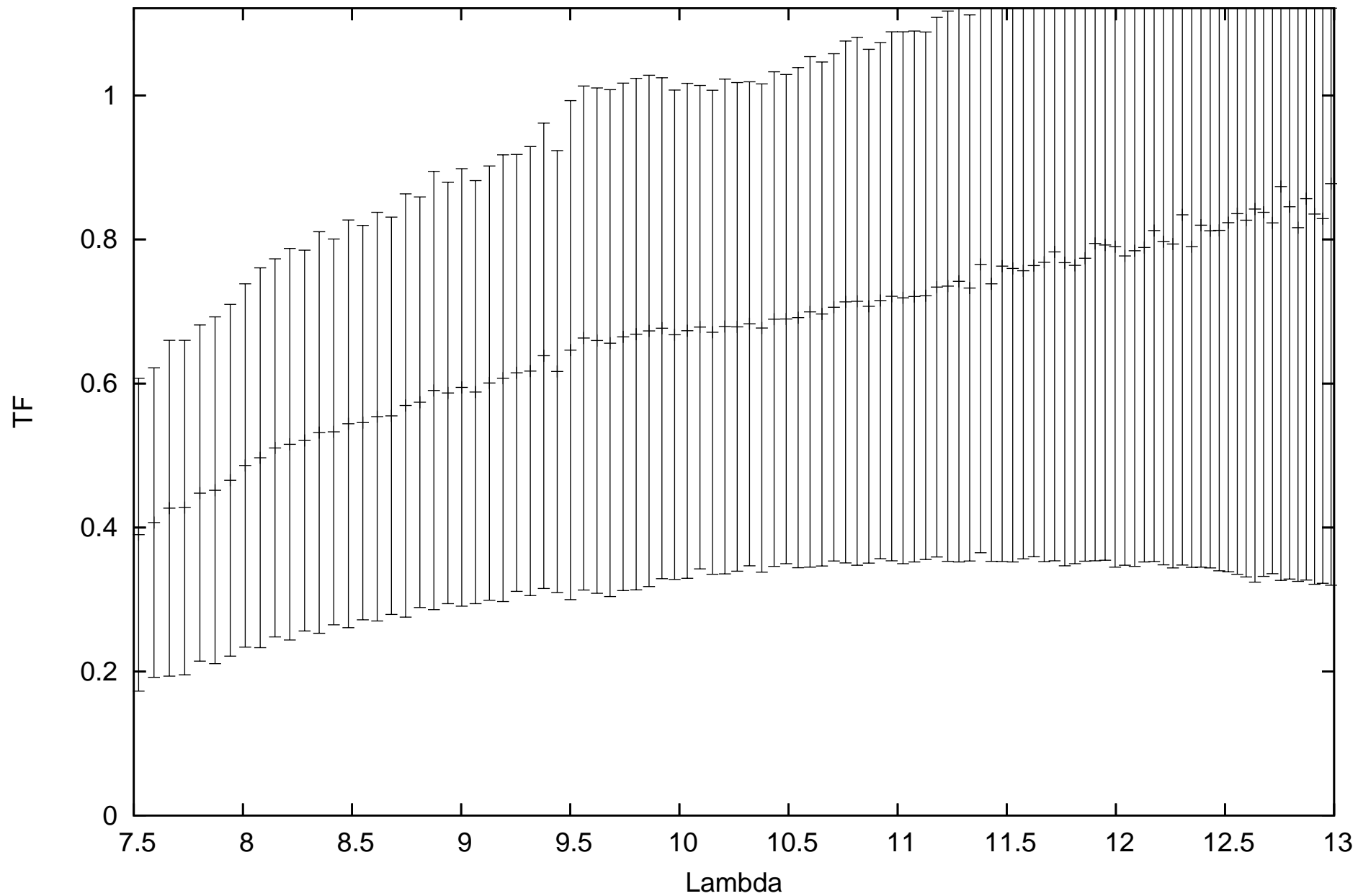
calHIP14135_flux-1.95419_diam12.27_r.MIDI.2011-10-04T07_15_23.000_K0J3
