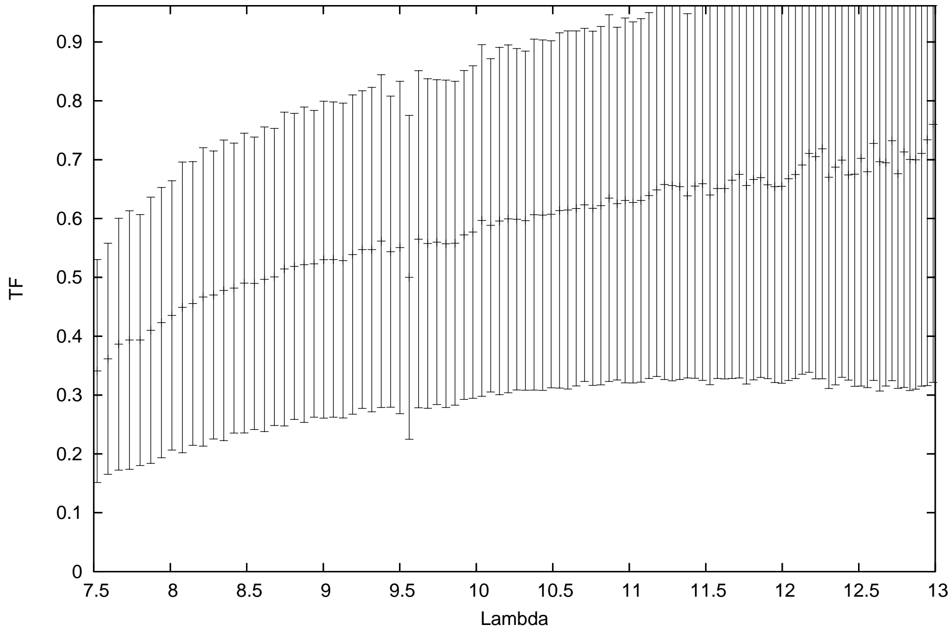
calHIP14135_flux-1.95419_diam12.27_r.MIDI.2011-10-04T07_34_56.000_J3K0
