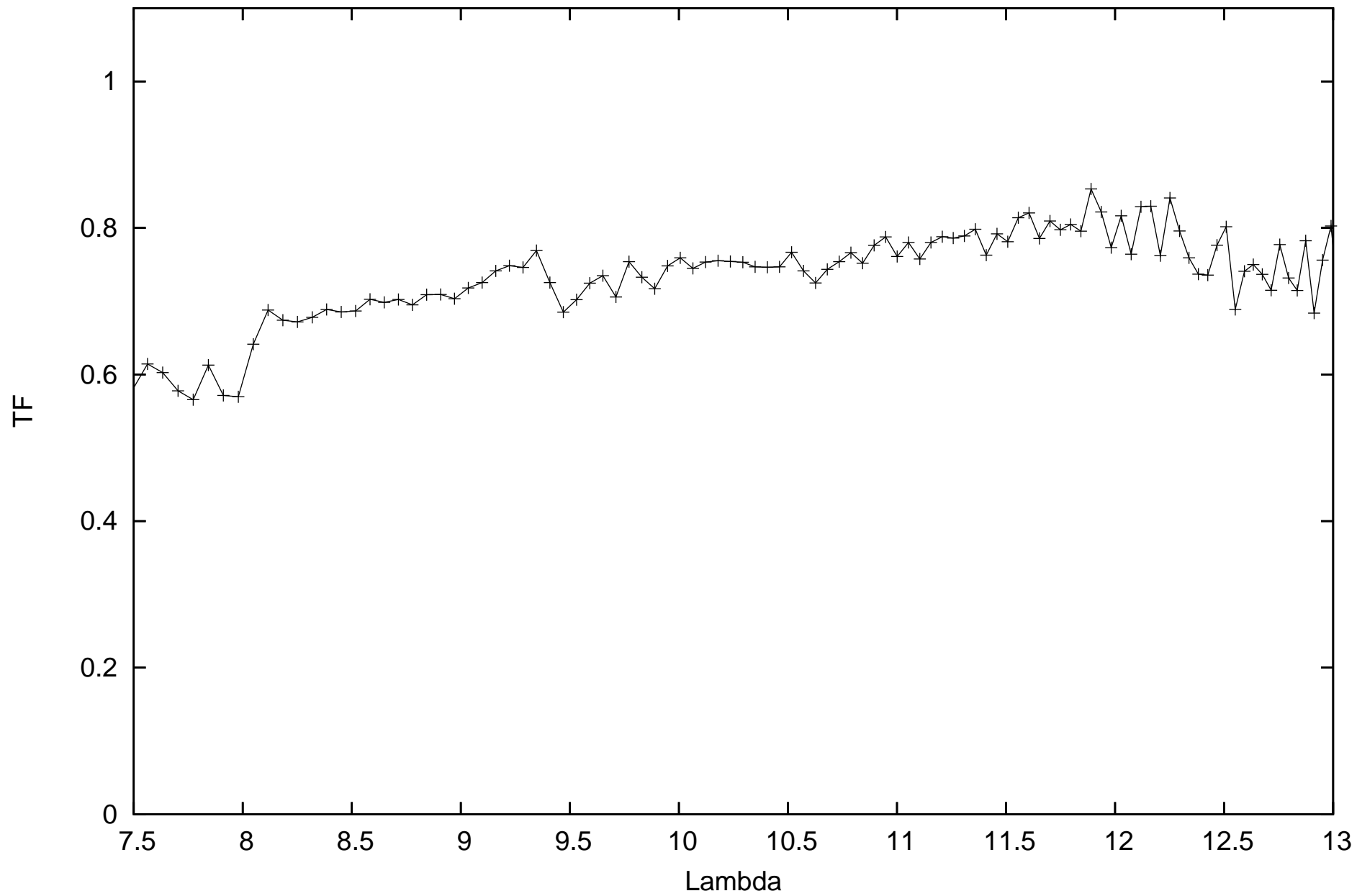
calHIP14135_flux-1.95419_diam12.27_r.MIDI.2011-10-21T07_36_09.970_C1A1
