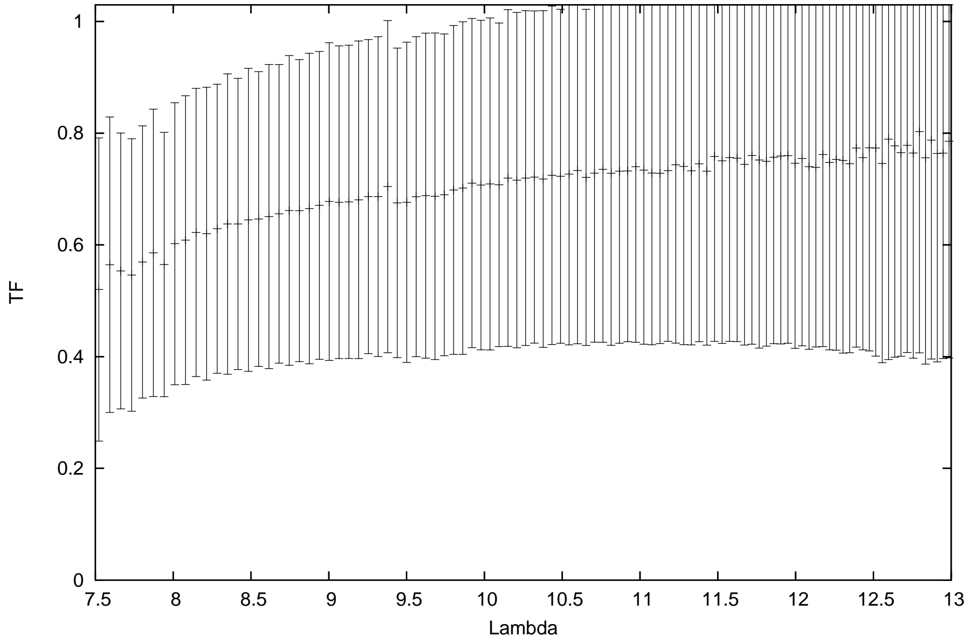
calHIP14135_flux-1.95419_diam12.27_r.MIDI.2011-11-01T05_48_13.000_G111
