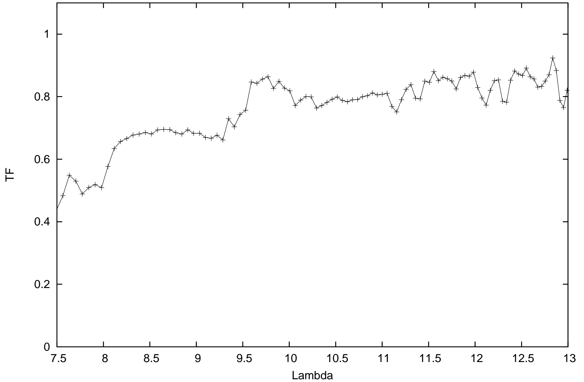
calHIP14135_flux-1.95419_diam12.27_r.MIDI.2011-11-04T03_33_16.135_H011
