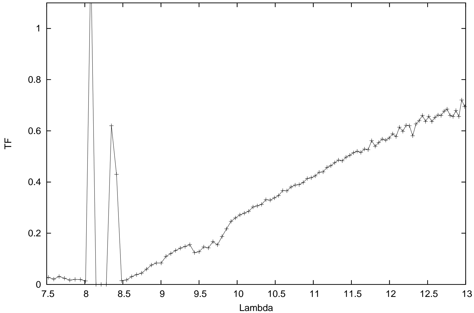
calHIP21421_flux-3.13927_diam20.4_r.MIDI.2011-10-02T08_30_10.000_J3G1
