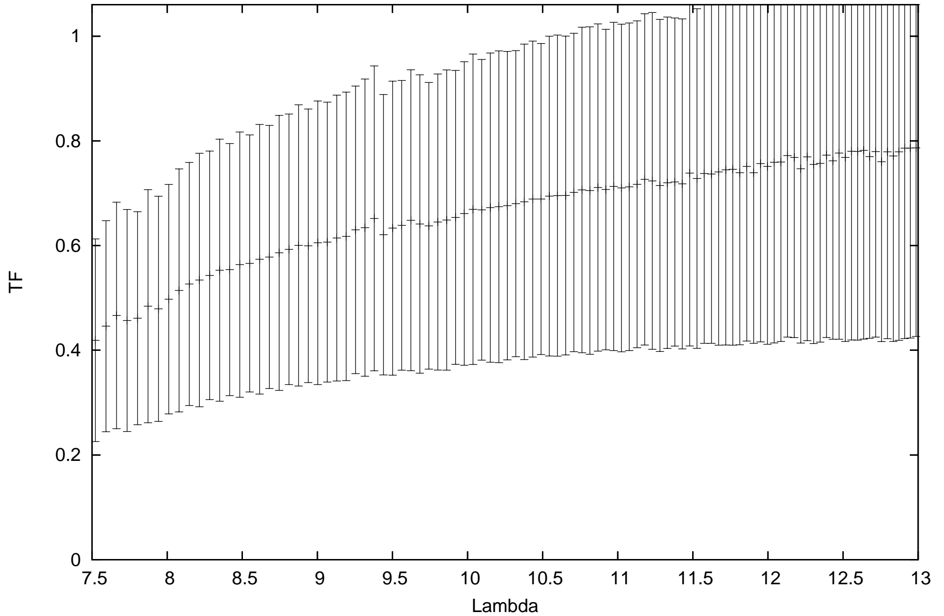
calHIP21421_flux-3.13927_diam20.4_r.MIDI.2011-10-28T07_36_34.000_K011
