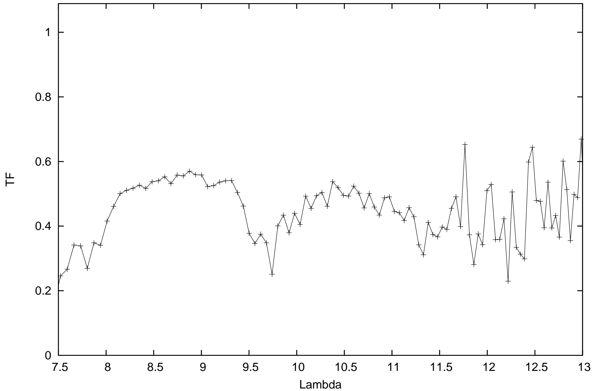
calHIP27628_flux0.355579_diam3.75_r.MIDI.2011-10-03T09_32_30.000_J3G1
