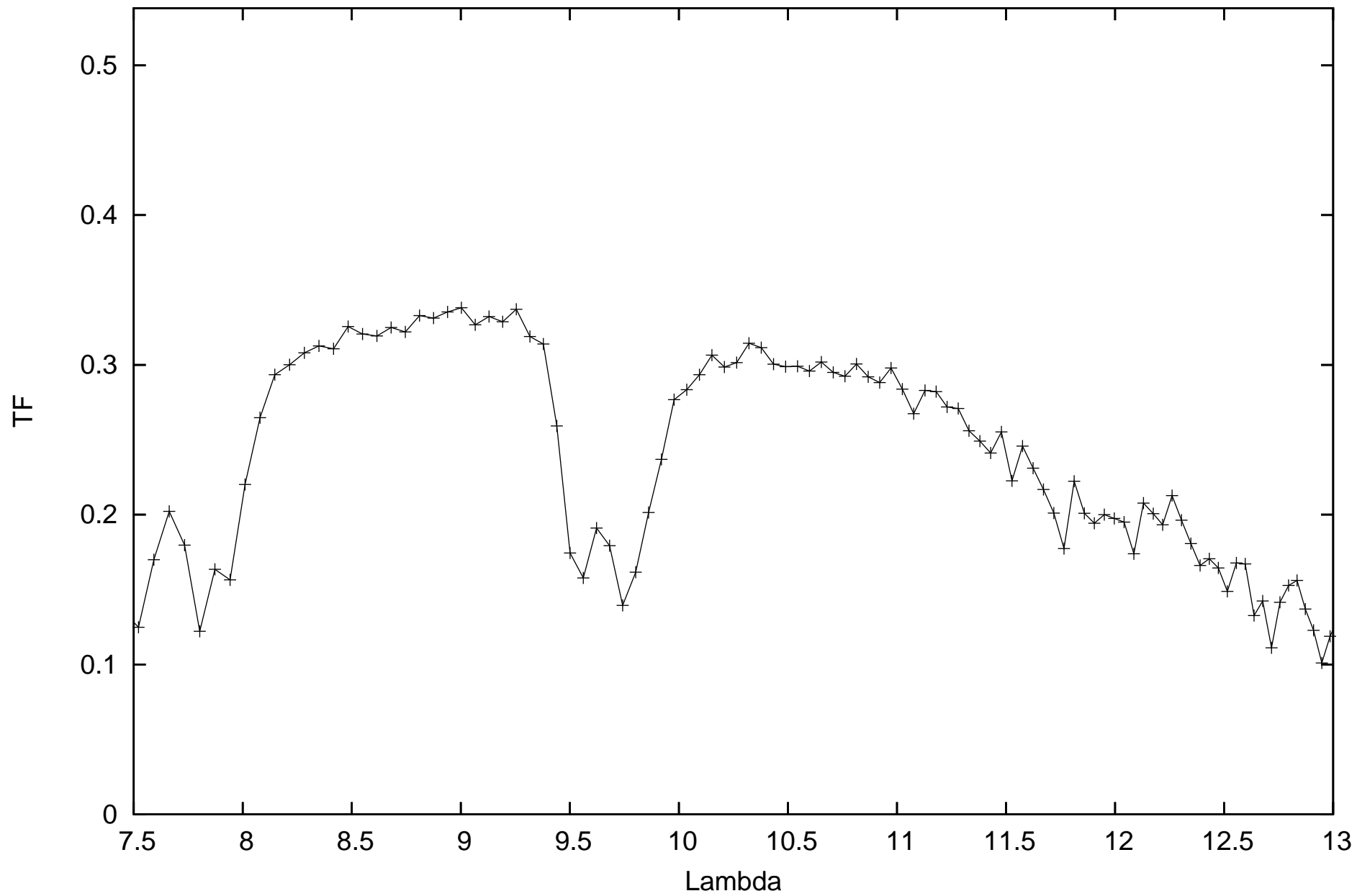
calHIP3419_flux-0.47009_diam5.23_r.MIDI.2011-12-04T04_28_04.000_J3G1
